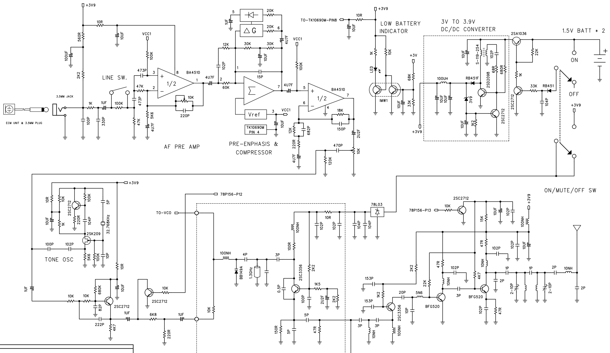
SCHEMATIC DIAGRAM UHF BAND PLL SYSTEM WIRELESS TRANSMITTER MODEL : UT-16A
