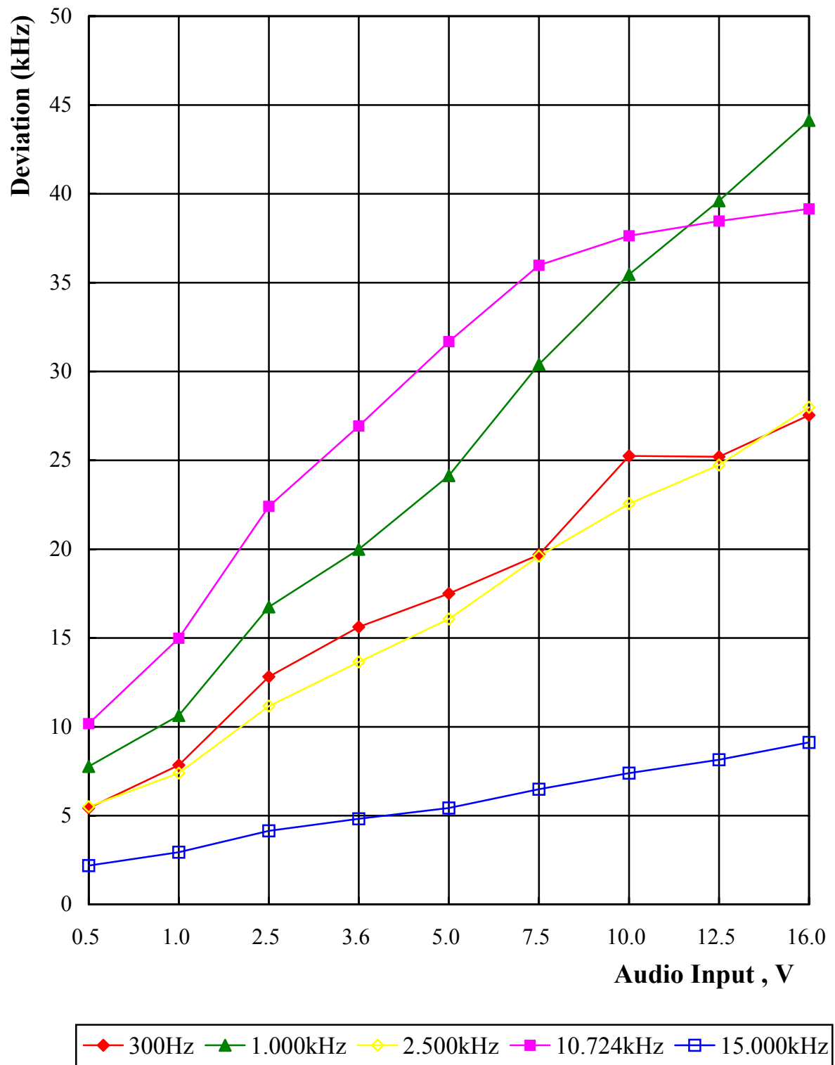
Chart 4.1 Modulation Limiting Measurement Negative
