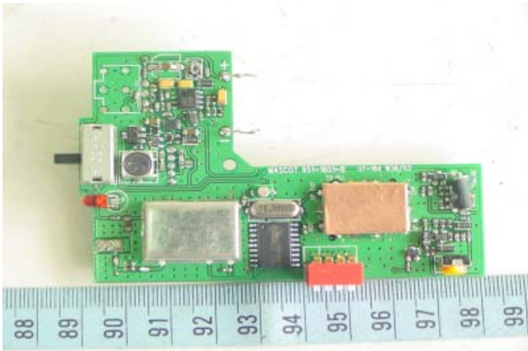
Component View of Main PCB
