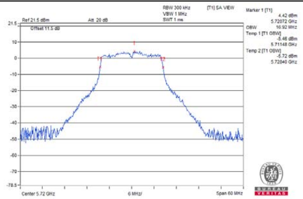
802.11ac (VHT20) / Chain 1 / CH 144
