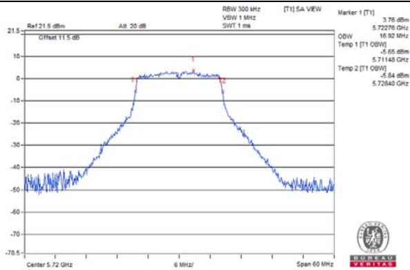
802.11ac (VHT20) / Chain 0 / CH 144
