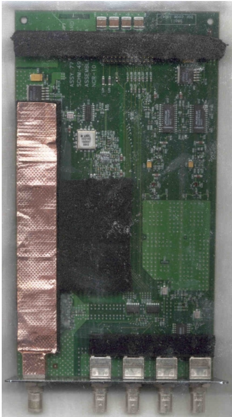
Photo 10. EUT, CBS II, Transceiver Board, Bottom View
