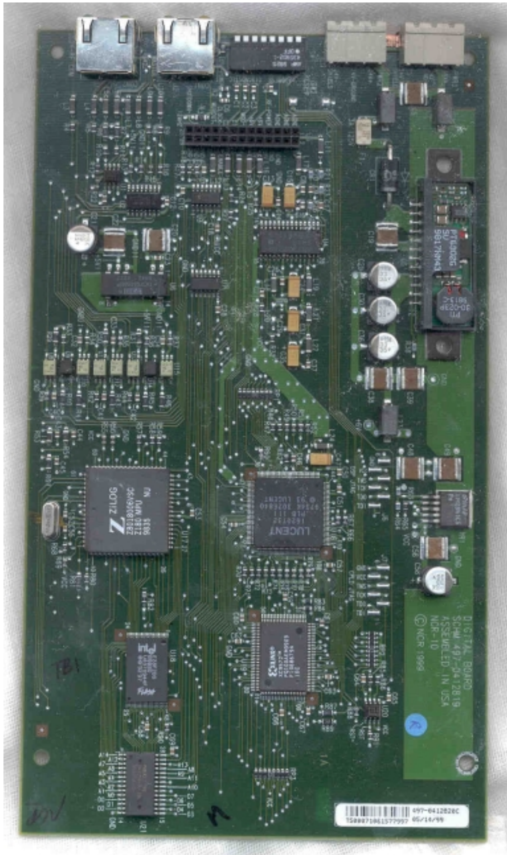
Photo 7. EUT, CBS II, Digital Board, Top View
