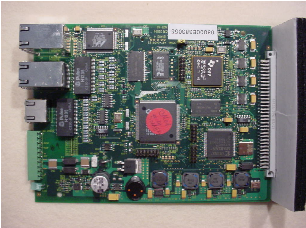
Figure 3: EUT DSP Board
