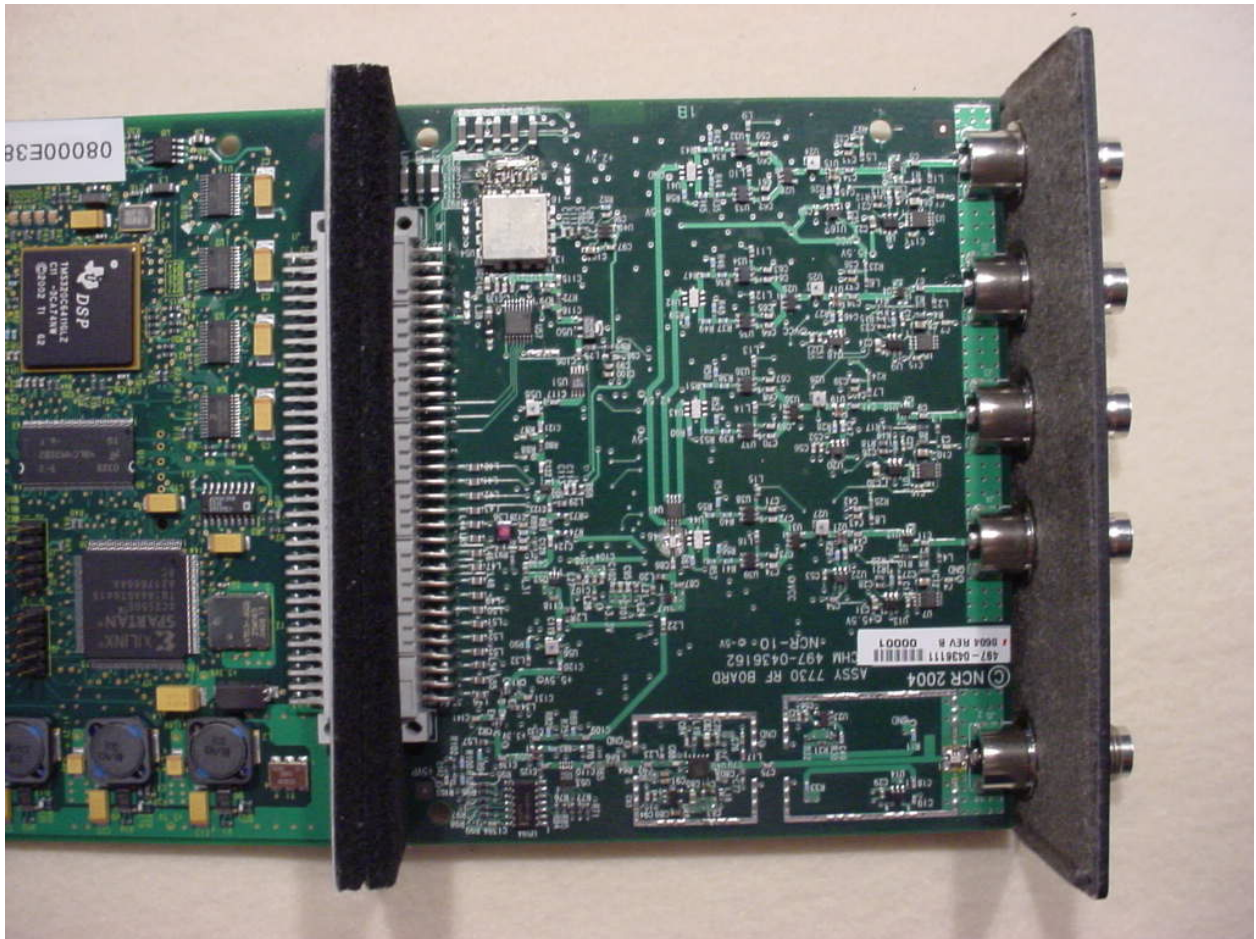
Figure 4: EUT Radio Board
