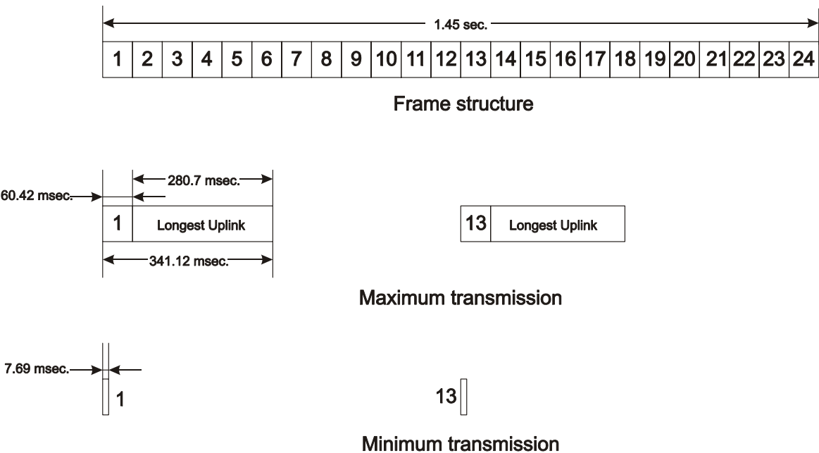
Fig. 3, System timing
