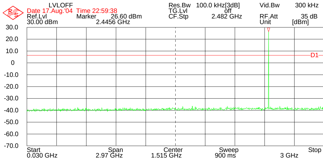
Figure 5: Mid Channel 30 – 3000 MHz
