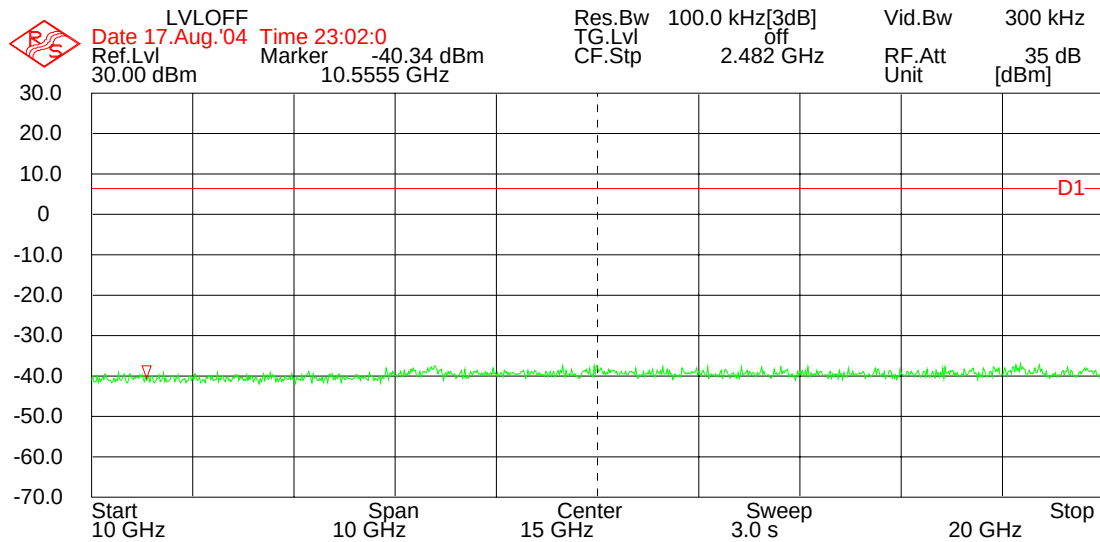
Figure 7: Mid Channel 10 – 20 GHz
