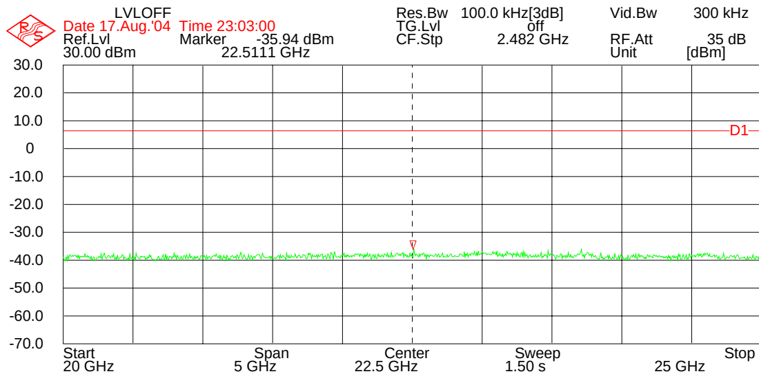
Figure 8: Mid Channel 20 – 25 GHz
