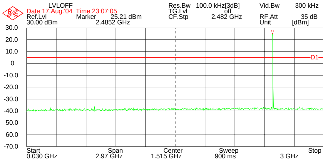
Figure 9: High Channel 30 – 3000 MHz
