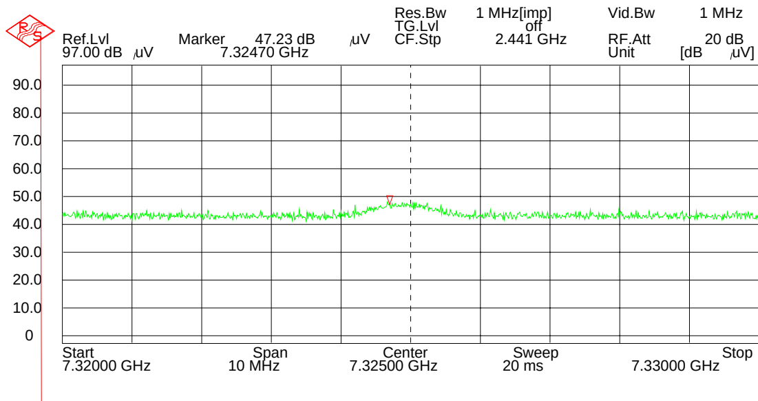
Figure 5: Mid Channel Vpol Peak 7325 MHz
