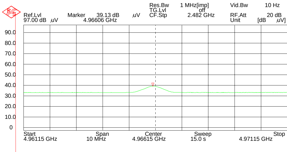
Figure 8: High Channel Hpol Average 4966.2 MHz
