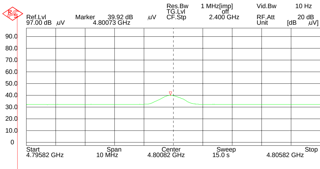
Figure 2: Low Channel Hpol Average 4800.8 MHz
