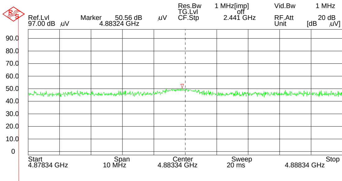
Figure 3: Mid Channel Hpol Peak 4883.3 MHz
