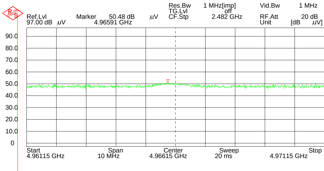
Figure 7: High Channel Hpol Peak 4966.2 MHz
