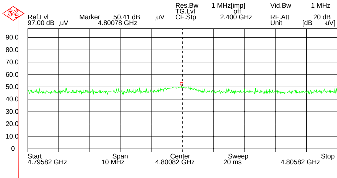
Figure 1: Low Channel Hpol Peak 4800.8 MHz
