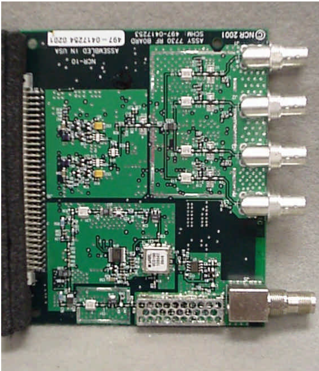
Photo 11. EUT, CBS Transceiver Board, Top View
