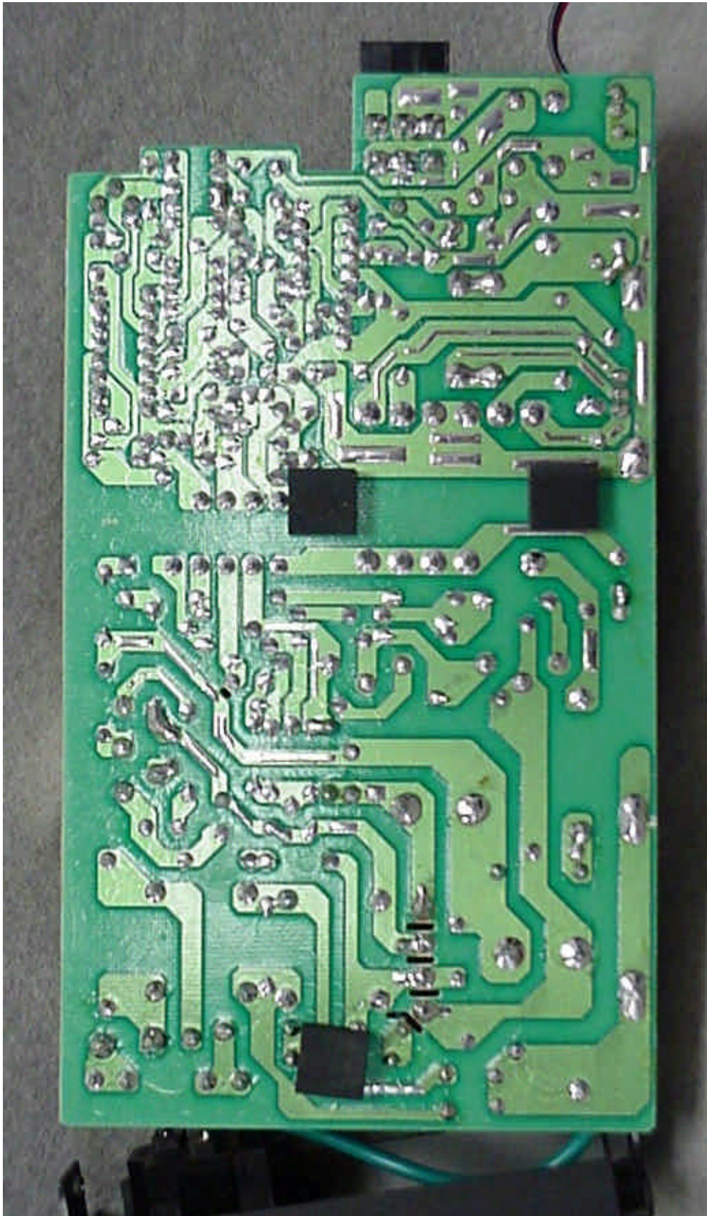
Photo 4. EUT, Power Supply Bottom View of Board
