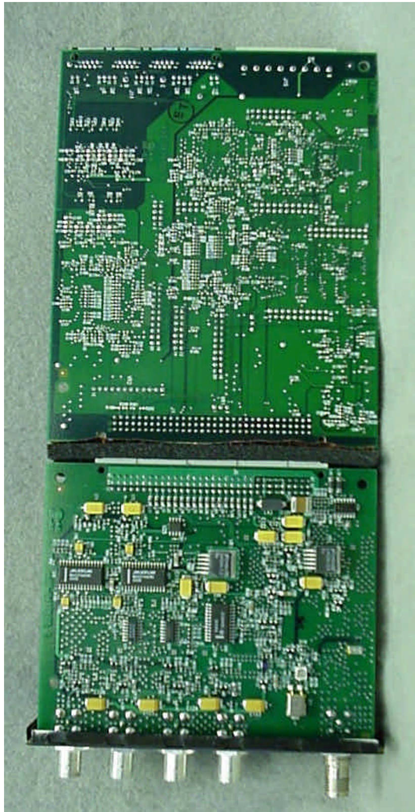
Photo 8. EUT, Bottom View of CBS Removed From Case
