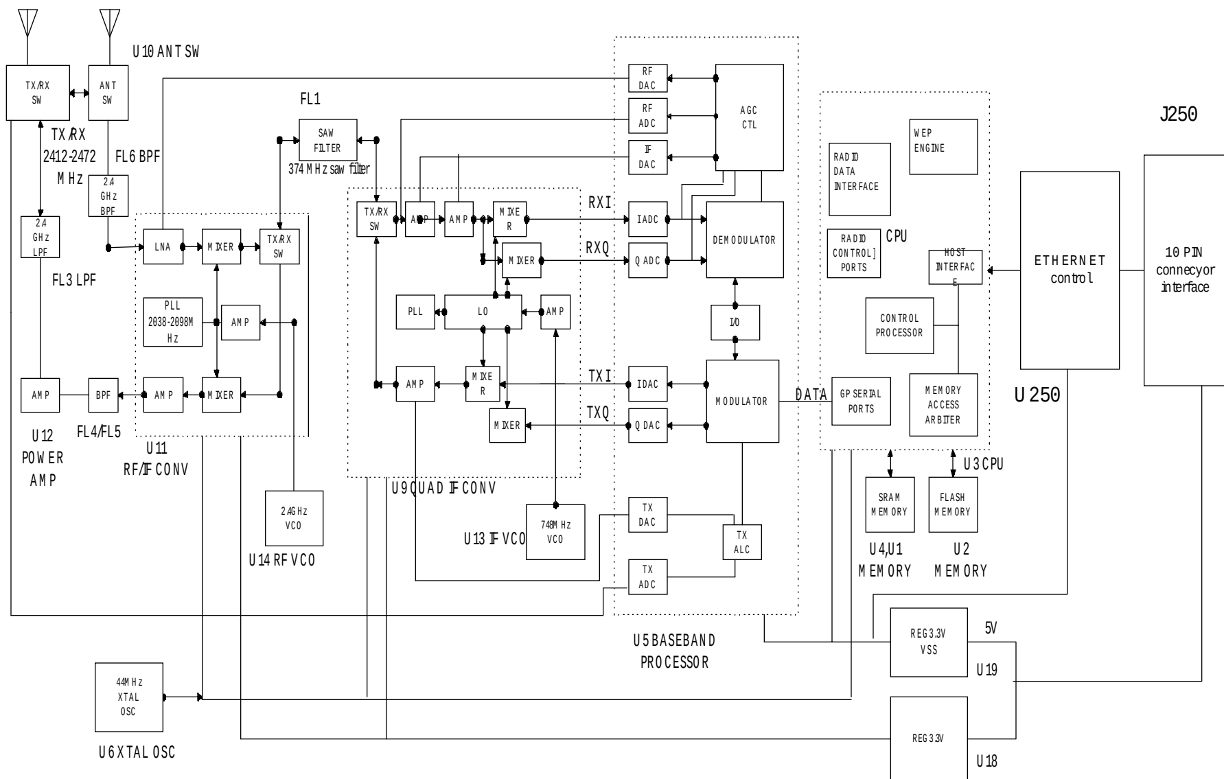
WX1513 BLOCKDIAGRAM
