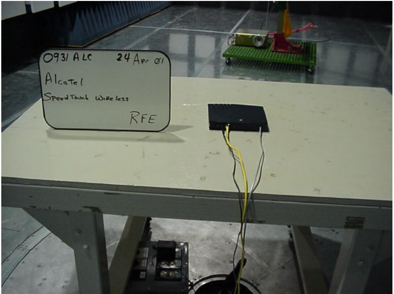
Figure 2 - Preliminary Radiated Emissions Test Setup (Chamber - Back)
