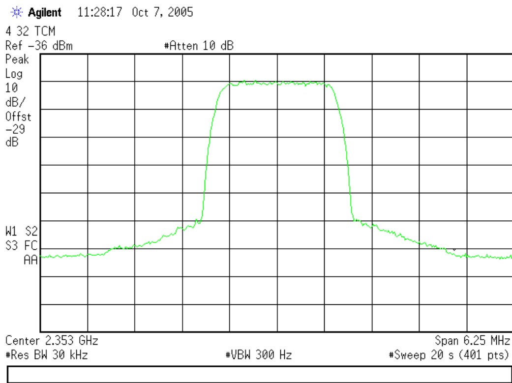
FIGURE 1. Typical Spectrum
