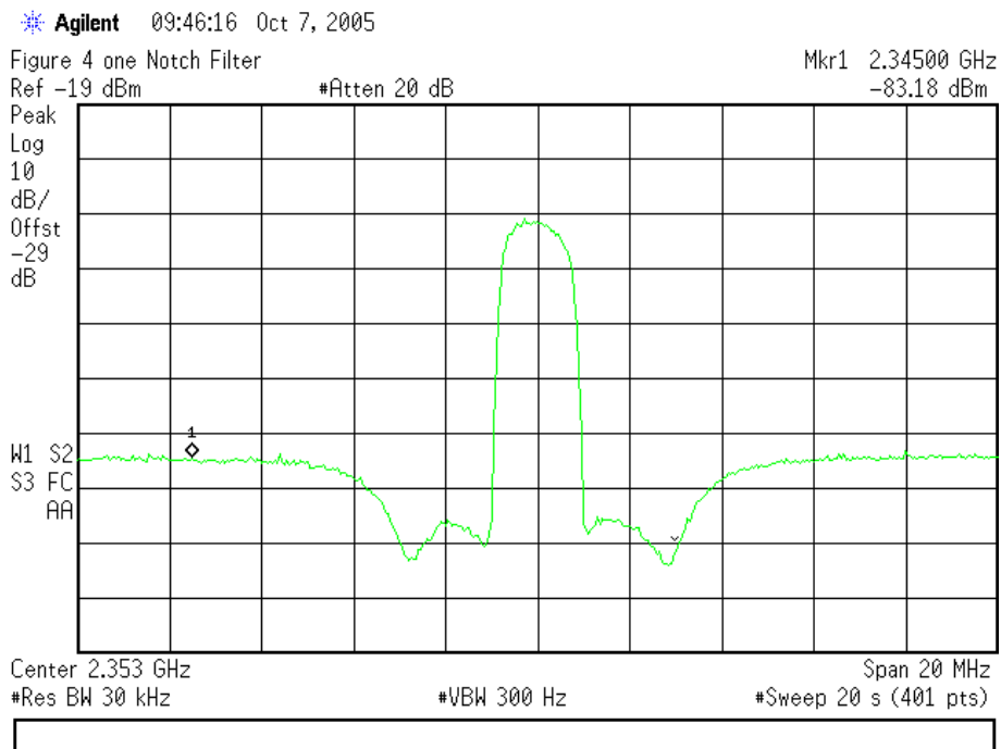
FIGURE 4. Typical Notch Filter
