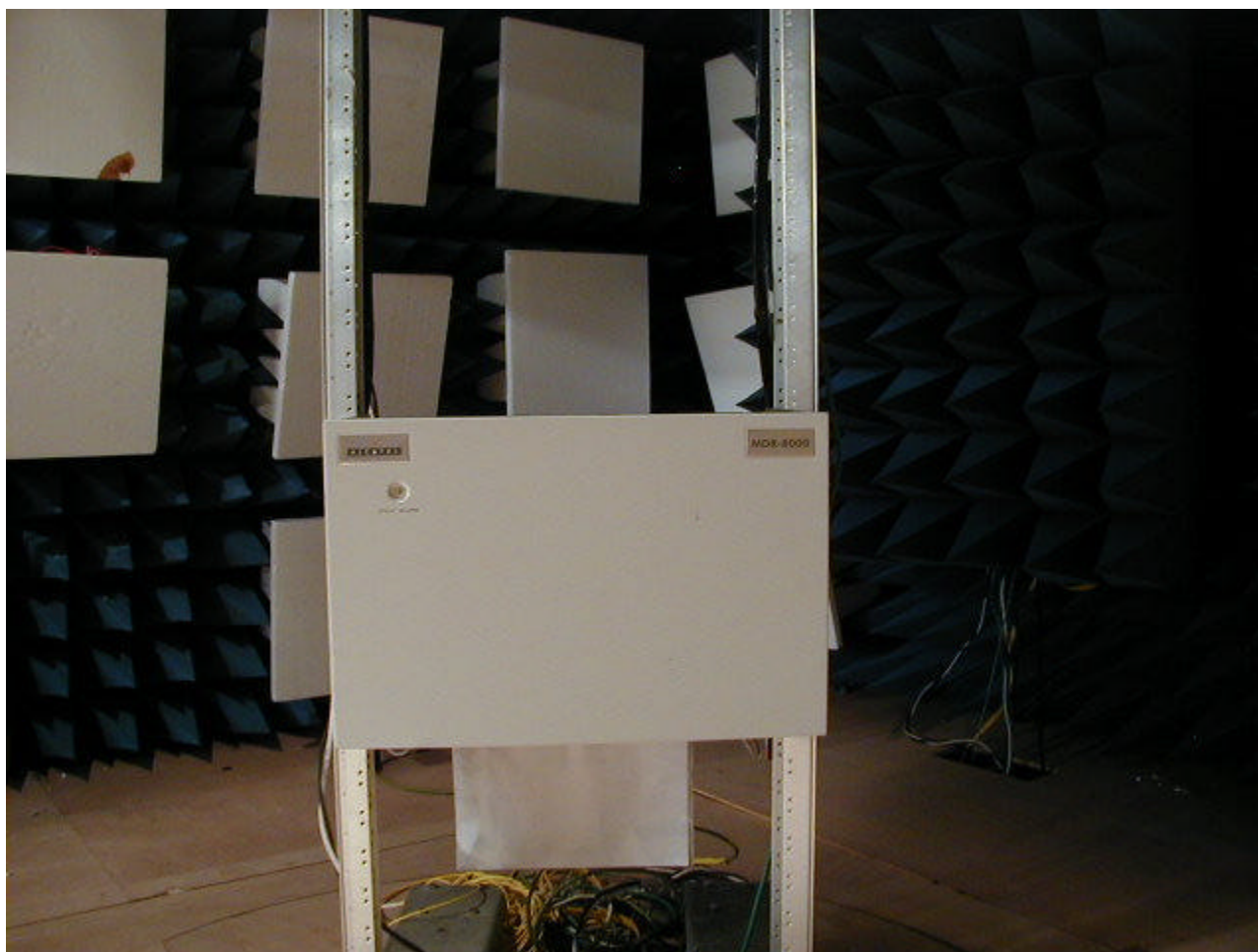
MDR-8X05u-XX radio mounted in a rack with cover on.
