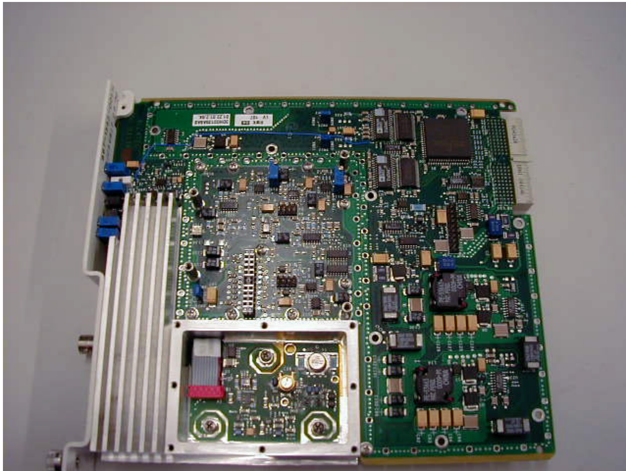
Transmitter (Biasing and Low Frequency Circuitry)
