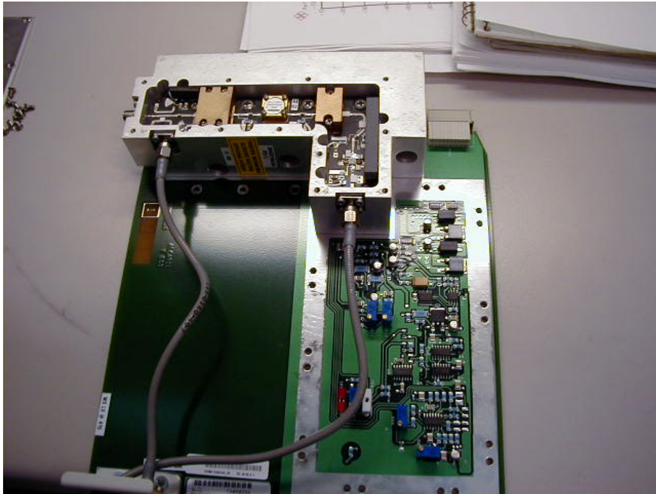
Power Amplifier (Front view, RF and Biasing Sections)
