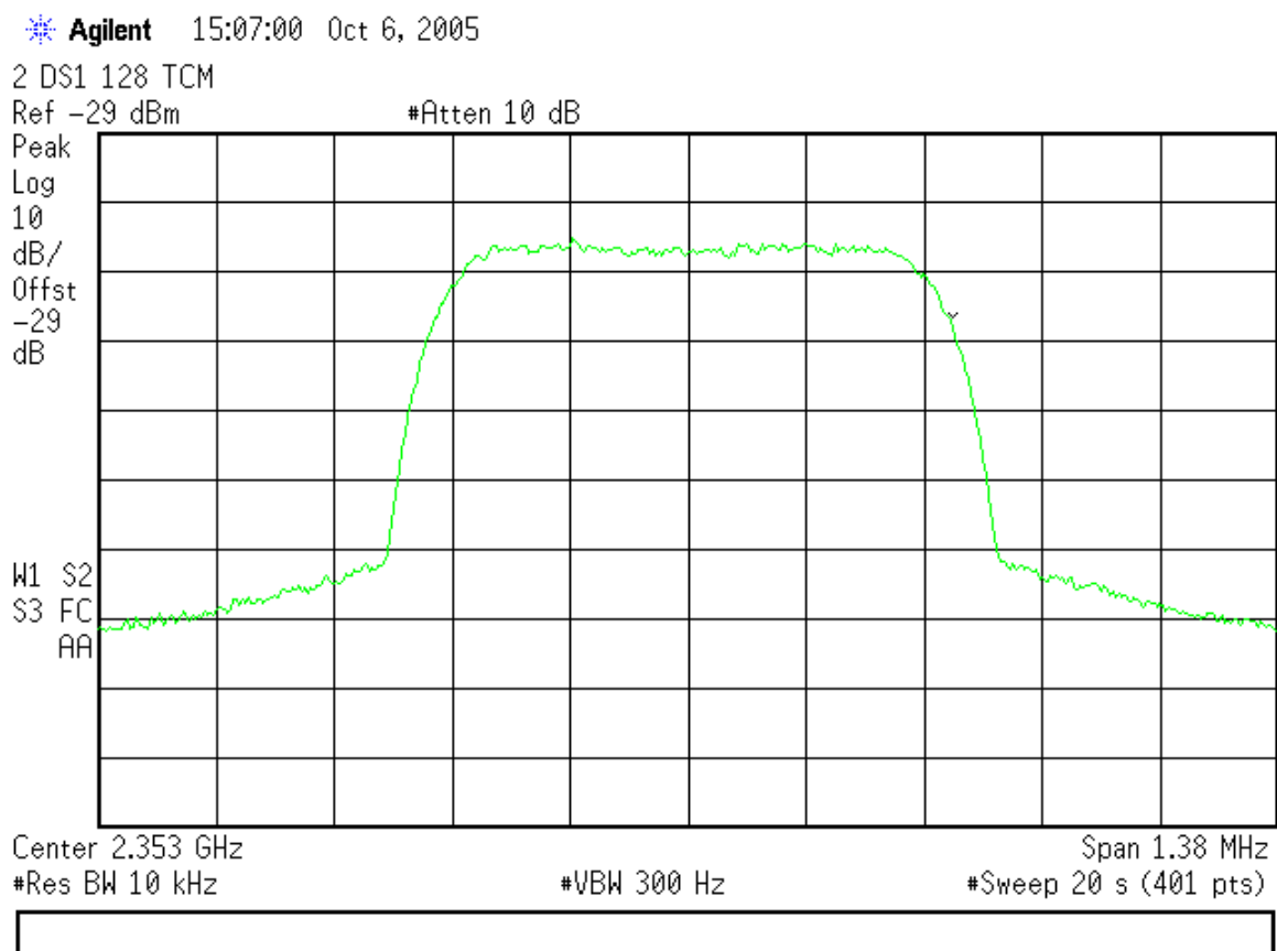
FIGURE 1. Typical Spectrum
