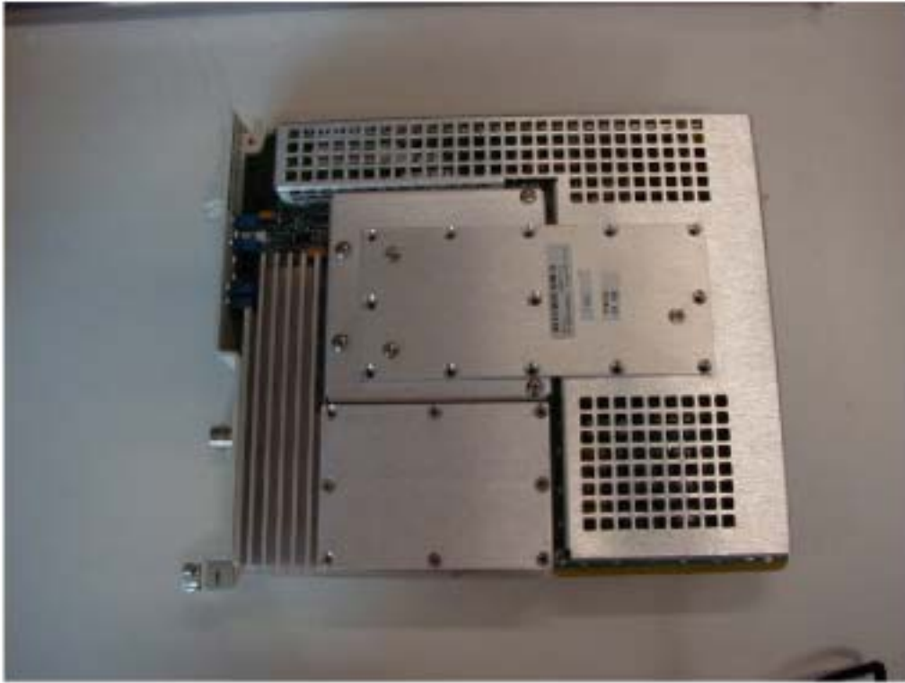
Transmitter (cover view)
