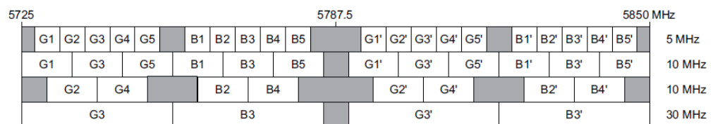
Figure 66 Frequency plan 9558HC: 5.725 to 5.850 GHz unlicensed band (FCC Part 15 and ISSED RSS-210)
