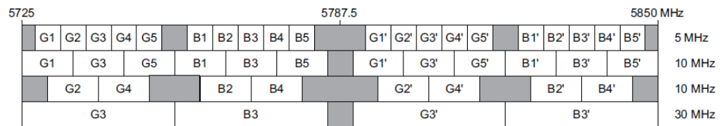
Figure 65 Frequency plan 9558HLC: 5.725 to 5.850 GHz unlicensed band (FCC Part 15 and ISSED RSS-210)
