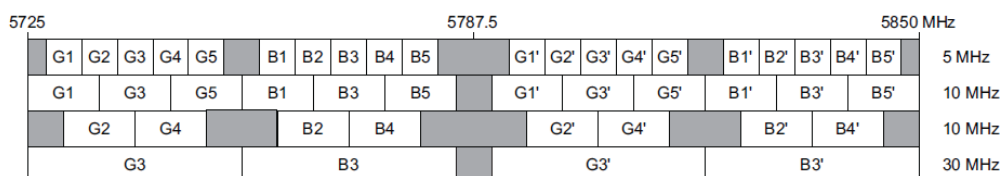
Figure 64 Frequency plan MPT-HL: 5.725 to 5.850 GHz unlicensed band (FCC Part 15 and ISSED RSS-210)
