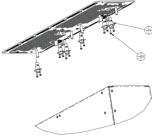
BMA-SMA CONNECTOR INSTALLATION
