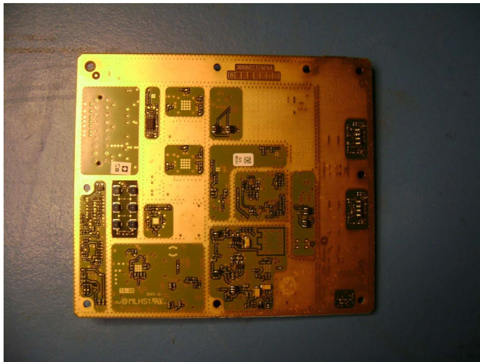
Transceiver Rx Diversity Board Back View
