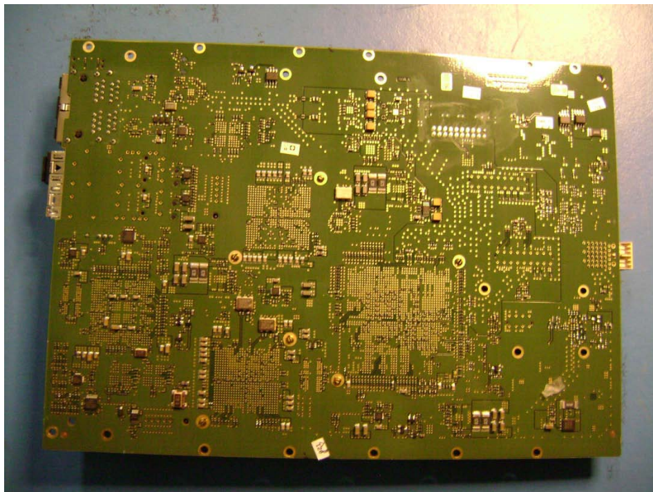
Transceiver Modem Board Back View
