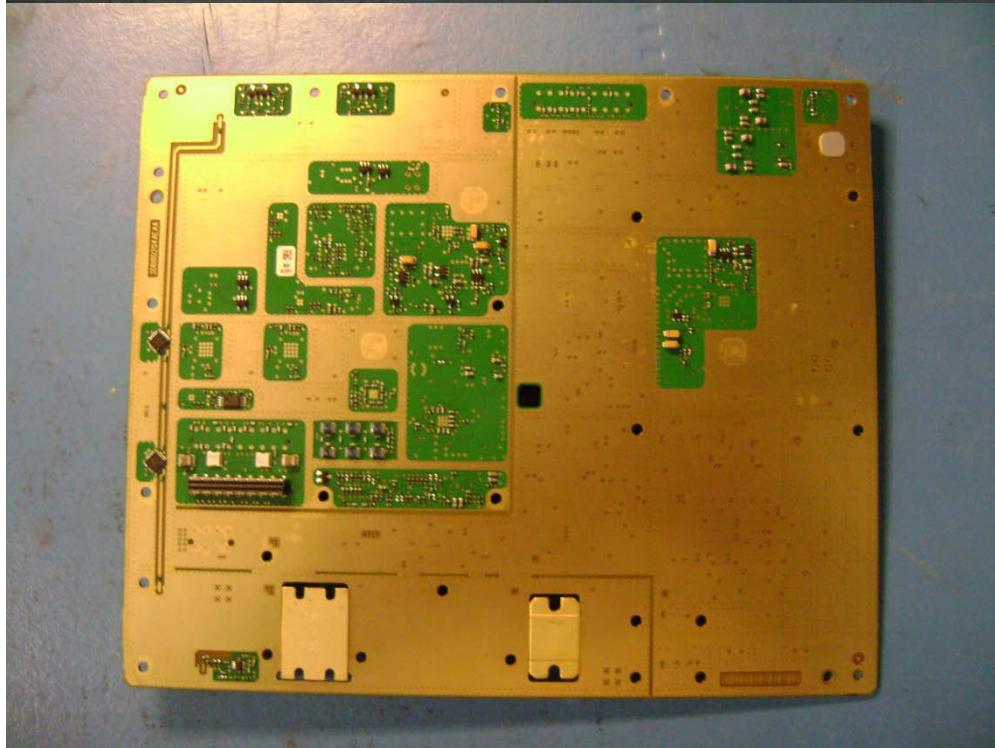
Transceiver RF Board Back View
