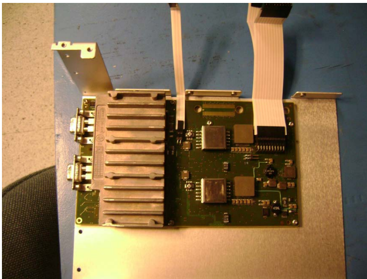
Transceiver Power Supply Board Front View
