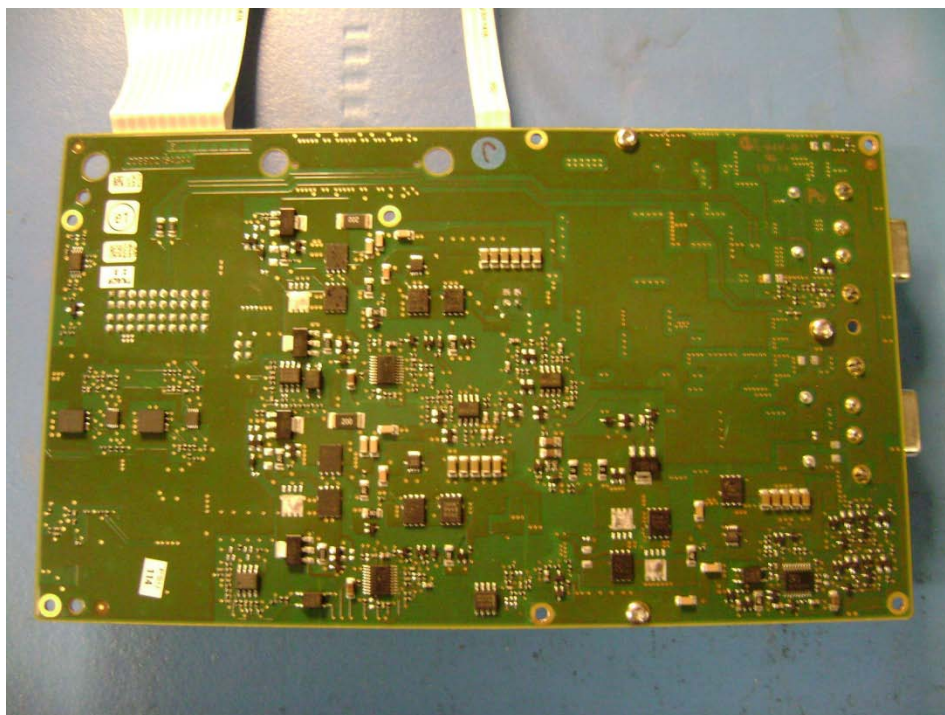
Transceiver Power Supply Board Back View
