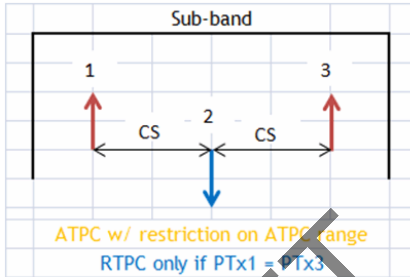
Figure 8.48 — ATPC with restriction
