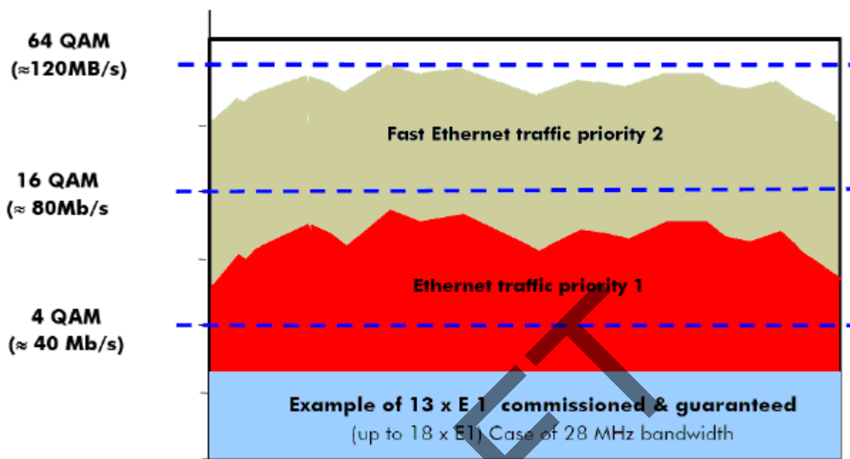
Figure 8.50 — Example of traffic 28MHz bandwidth and admission control
