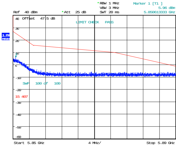
Figure 8.2-21: -Conducted spurious emissions 5.85-5.89 GHz, 10 MHz Channel BW, High channel
