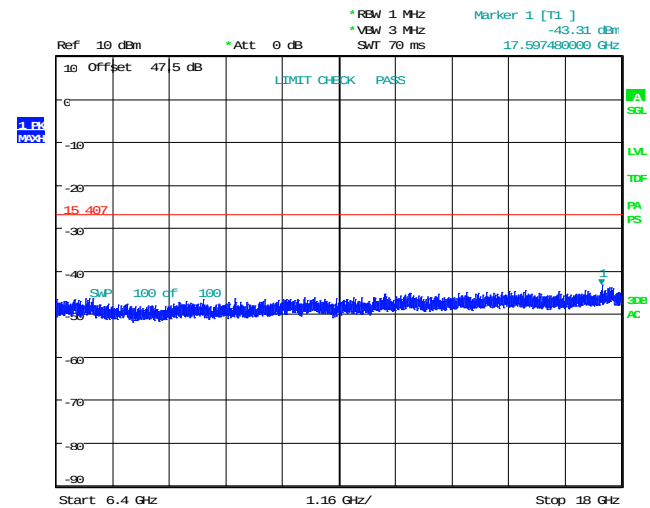
Figure 8.2-12: Conducted spurious emissions 6.4-18 GHz, 5 MHz Channel BW, Low channel
