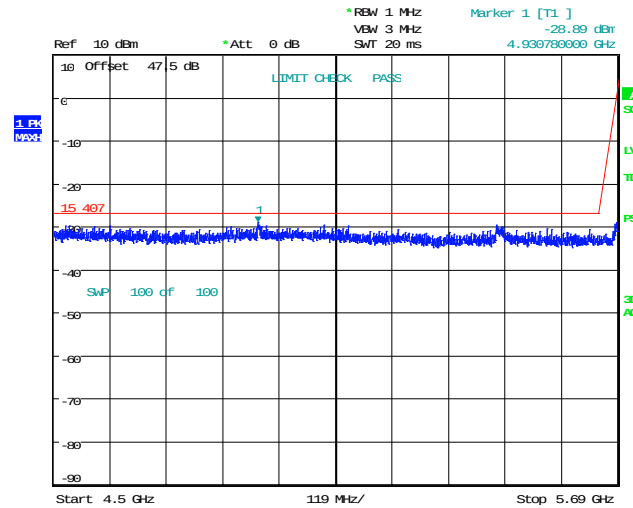
Figure 8.2-3: Conducted spurious emissions 4.5-5.69 GHz, 5 MHz Channel BW, Low channel
