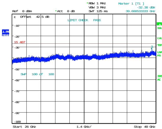
Figure 8.2-30: Conducted spurious emissions 26-40 GHz, 5 MHz Channel BW, High channel
