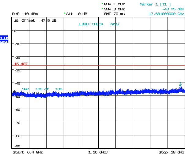
Figure 8.2-26: Conducted spurious emissions 6.4-18 GHz, 5 MHz Channel BW, High channel
