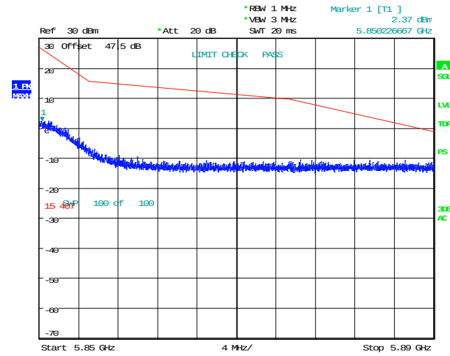
Figure 8.2-20: Conducted spurious emissions 5.85-5.89 GHz, 5 MHz Channel BW, High channel
