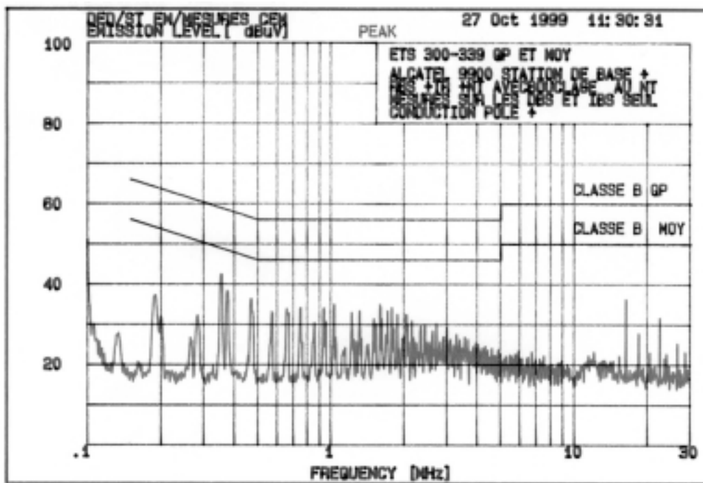
Exhibit 10 - Conducted Emissions on Positive Conductor
