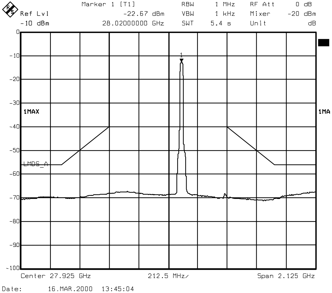
Exhibit 1 - Modulation Characteristics at 28020 MHz
