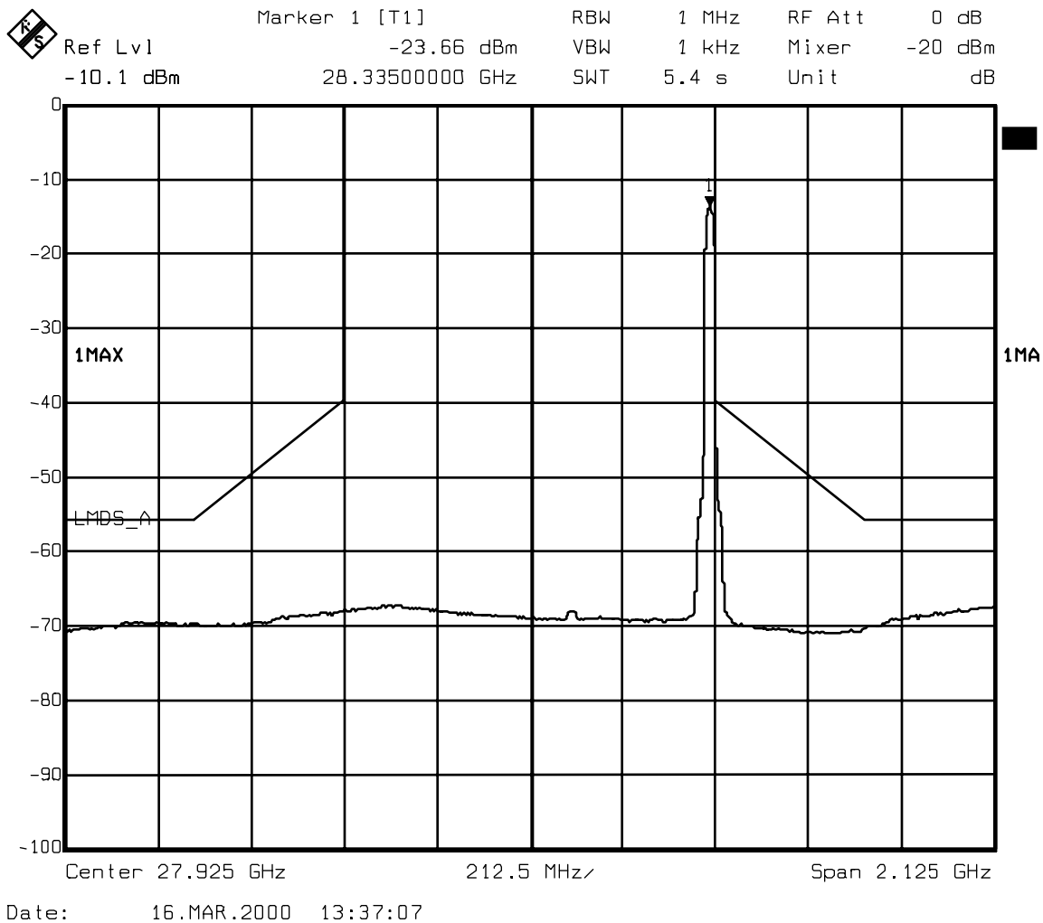
Exhibit 2 - Modulation Characteristics at 28335 MHz
