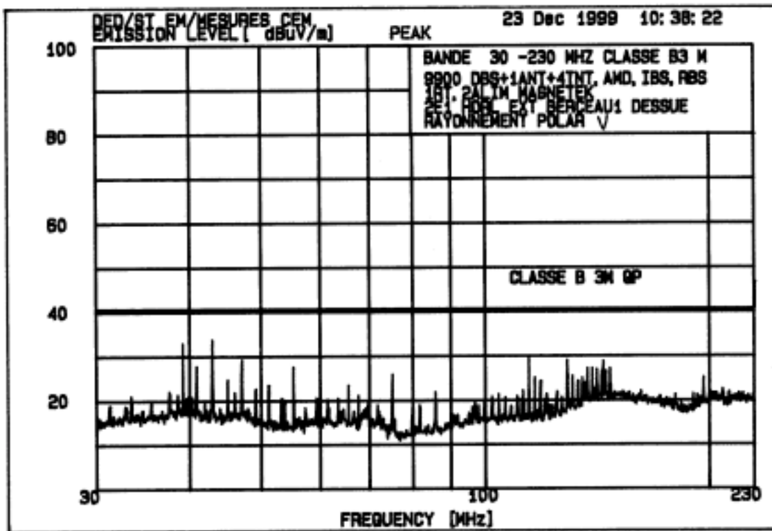
Exhibit 7 - Spurious Radiation (vertical)
