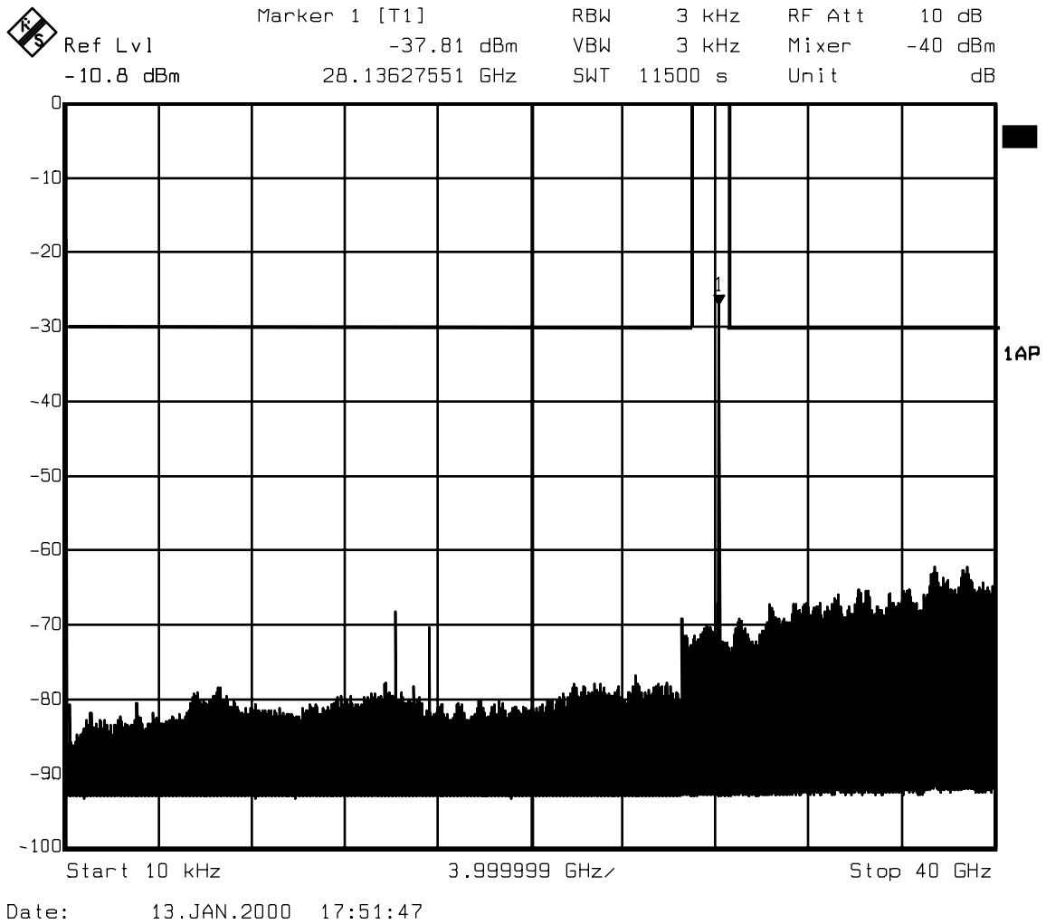
Exhibit 5 - Emissions at the Antenna Port
