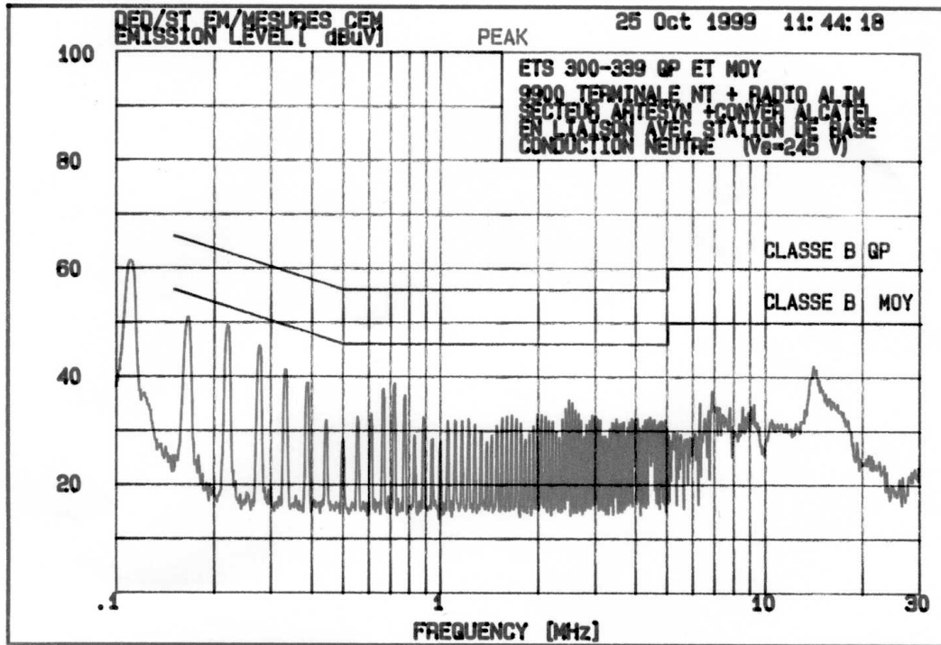
Exhibit 8 - Artesyn supply, neutral conductor @ 245V
