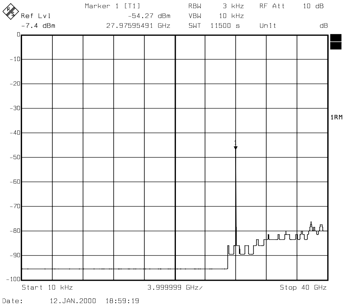
Exhibit 3 - Emissions at the Antenna Port
