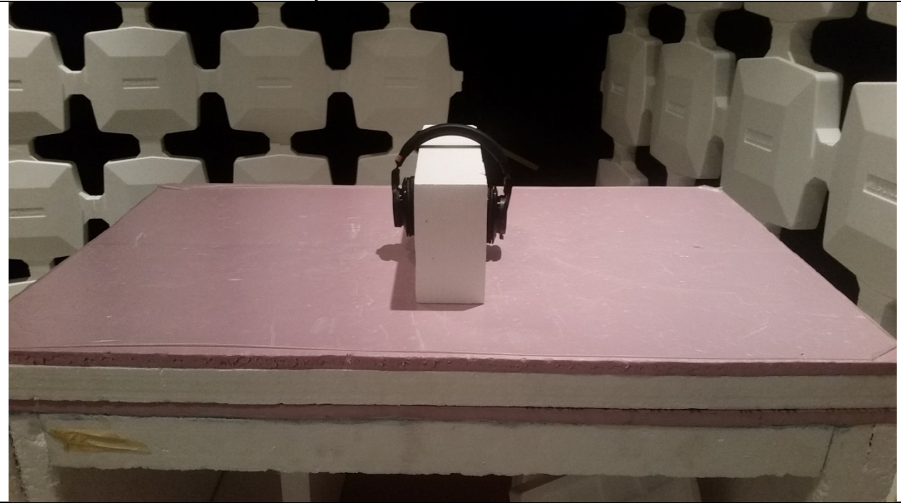
RADIATED TESTS: Final Setup Position
