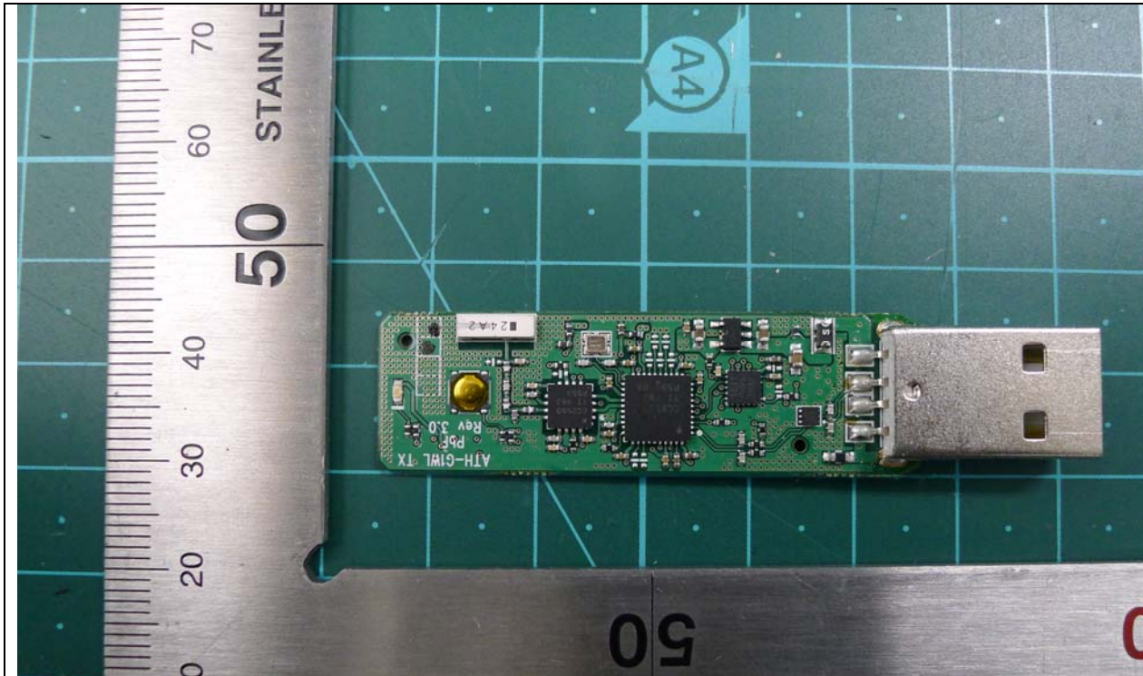
PCB Front
