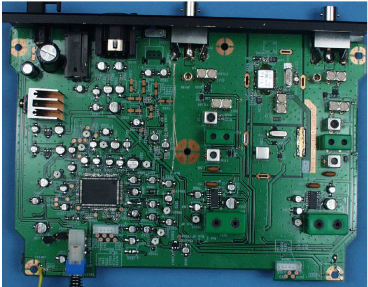
Circuit Board, Top View w/o Shield
