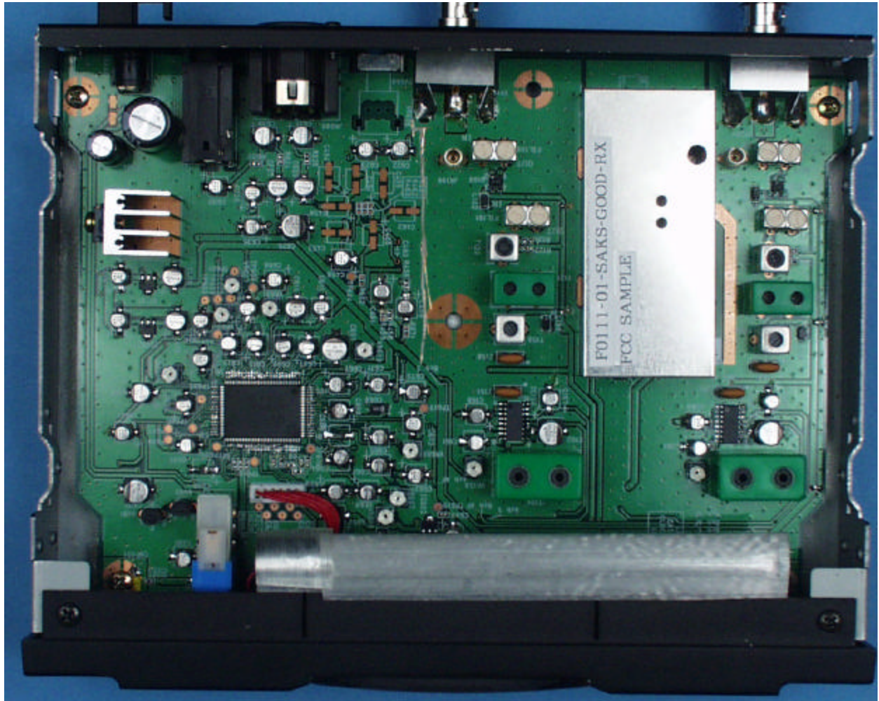
Circuit Board, Top View
