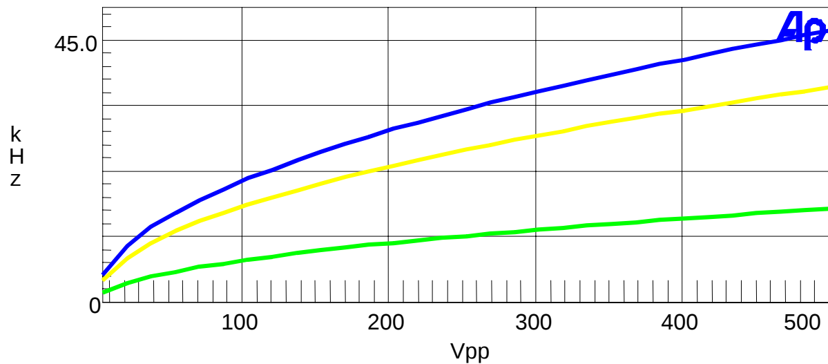
Modulation Limiting Plots: 15 KHz (Green), 3.0 KHz (Blue), and 300 Hz (Yellow)
