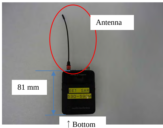
Photograph C1: Antenna position
