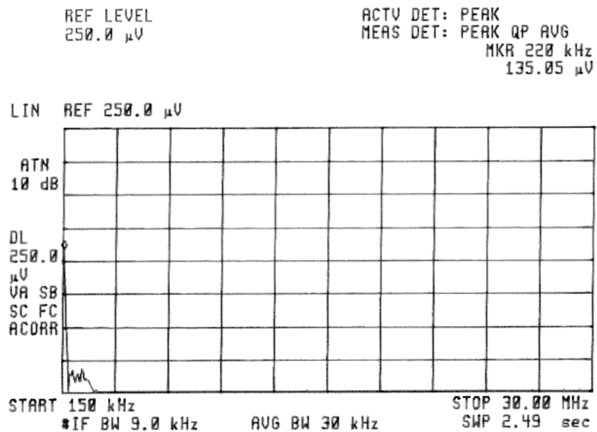
Figure 5.1.b Neutral Conducted-9V
