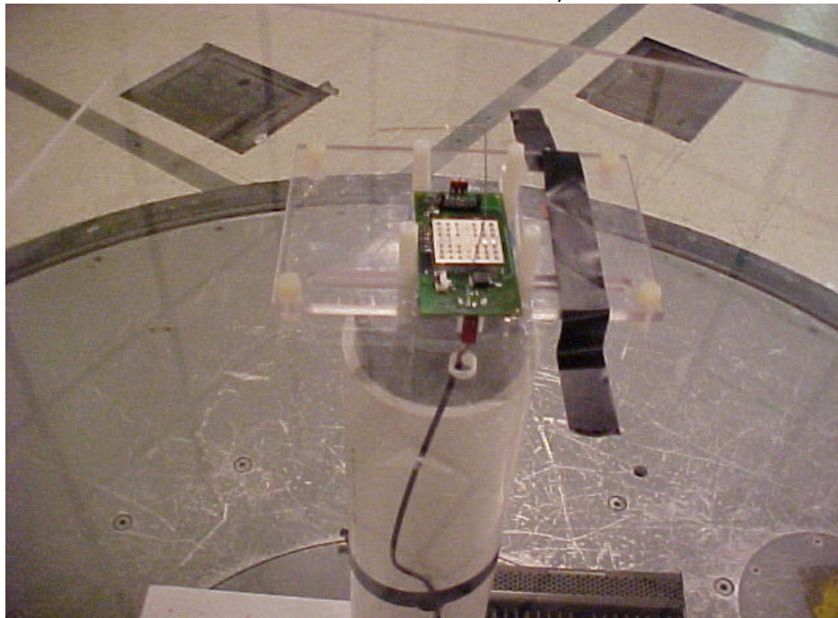
View of the EUT during Radiated Emission Testing in the 3 Meter FCC Listed Chamber, Antenna A
