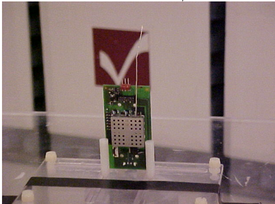
View of the EUT during Radiated Emission Testing in the 3 Meter FCC Listed Chamber, Antenna B
