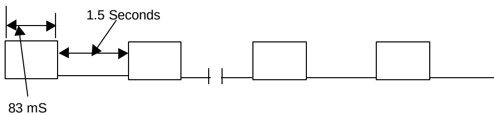
Transmit Burst Sequence Timing
