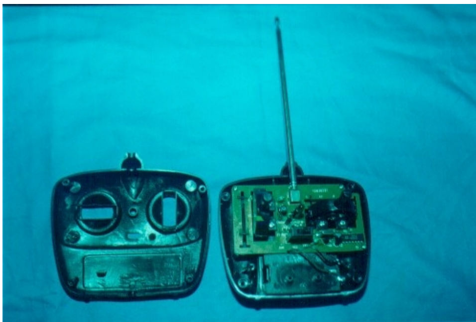
Figure 3. Inside of the Eut
