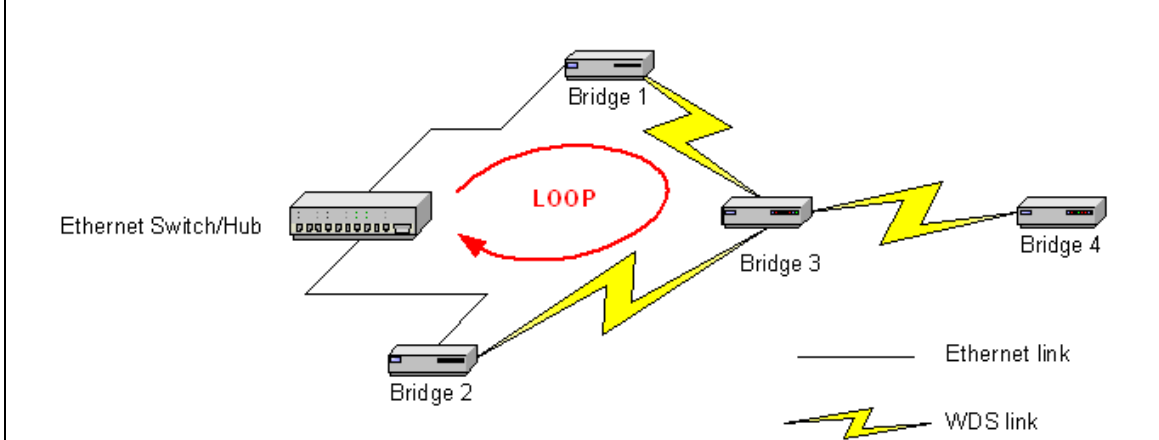
Fig. 12. Network topology containing a loop.
