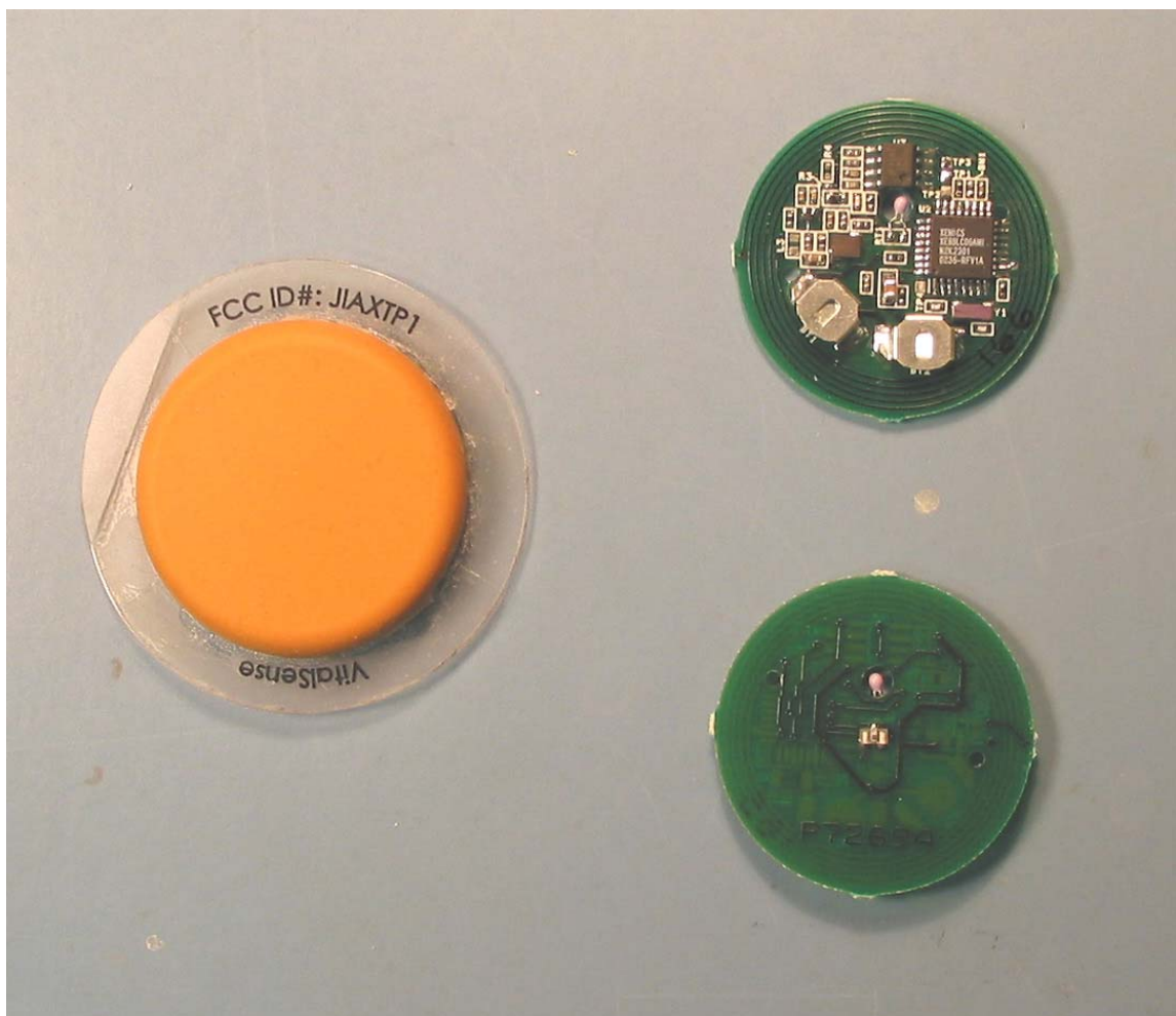
Figure 3: On the left is a photograph of the Dermal Patch Assembly with proposed FCC ID# label. On the right is the primary and secondary view of the Dermal Patch sensor subassembly.
