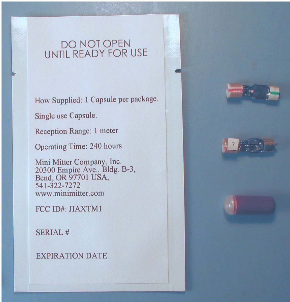
Figure 2: Photograph of Proposed Capsule Envelope Label showing FCC ID#. The FCC label ID# is on the row third from the bottom. A photograph of the capsule sensor assembly and subassembly is placed next to the envelope for size comparison.
