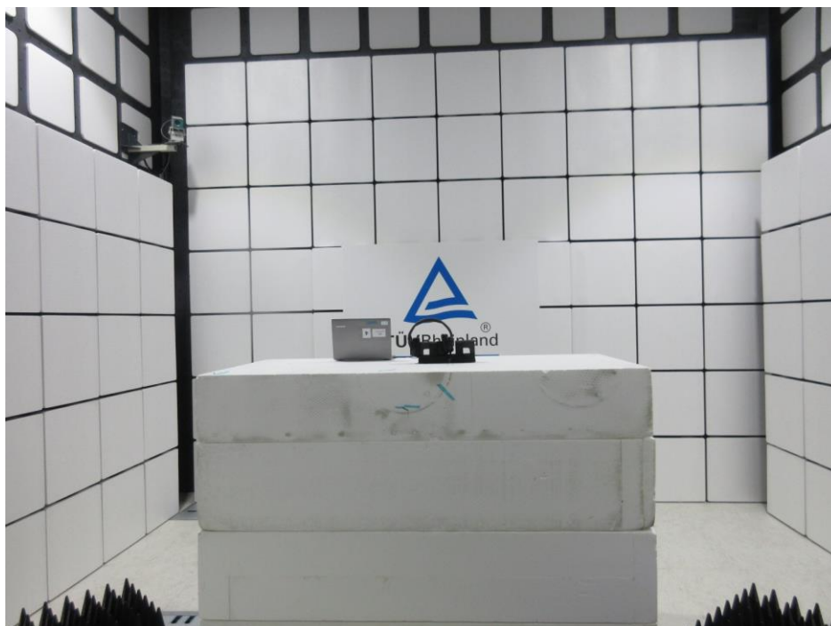
Photograph 2: Set-up for Spurious Emissions (Z Axis Orientation Pre-test)
