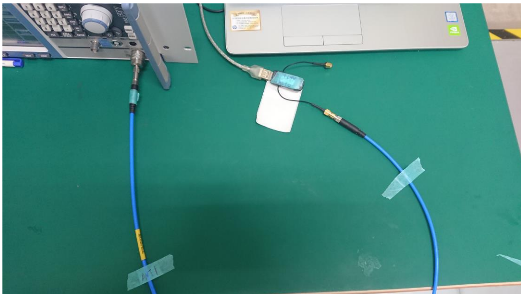
Photograph 5: Set-up for Conducted Testing
