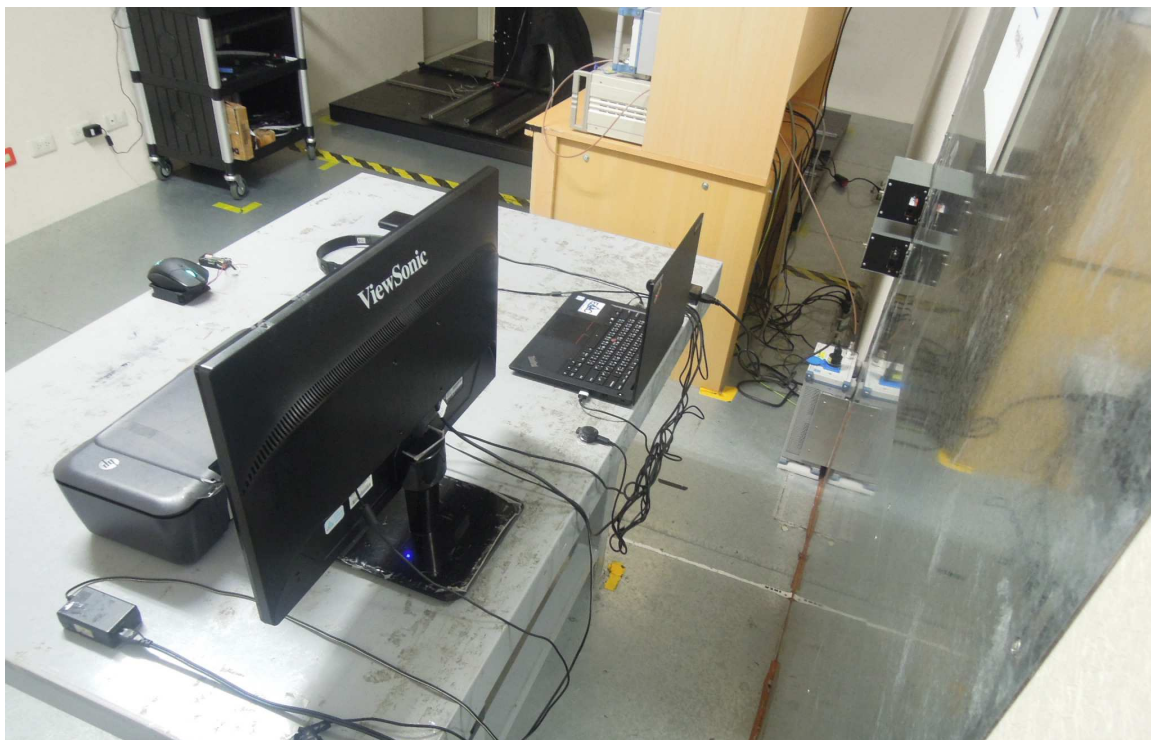
Photograph 5: Set-up for for Mains Conducted testing Back
