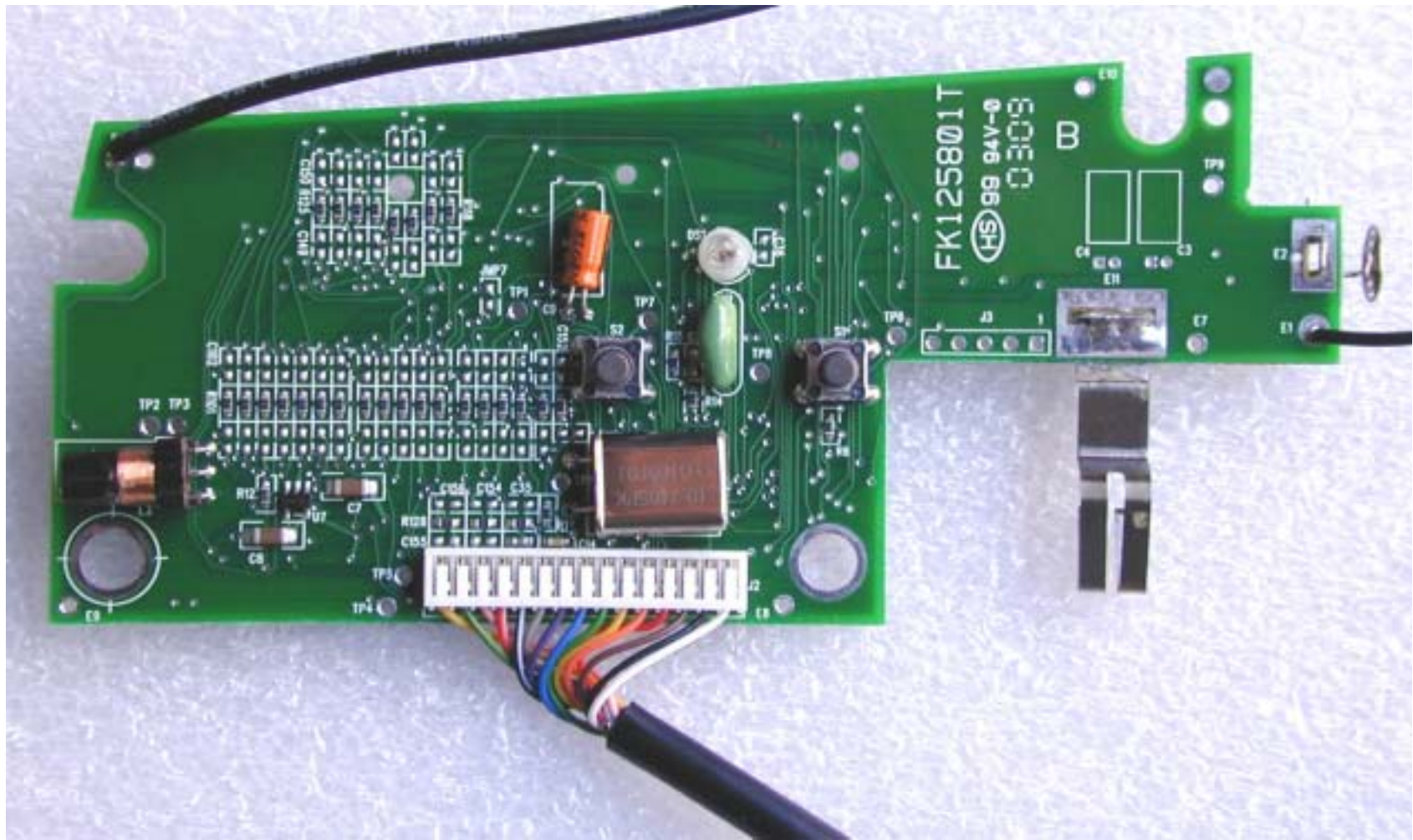
Bottom Side of Transmitter Board
