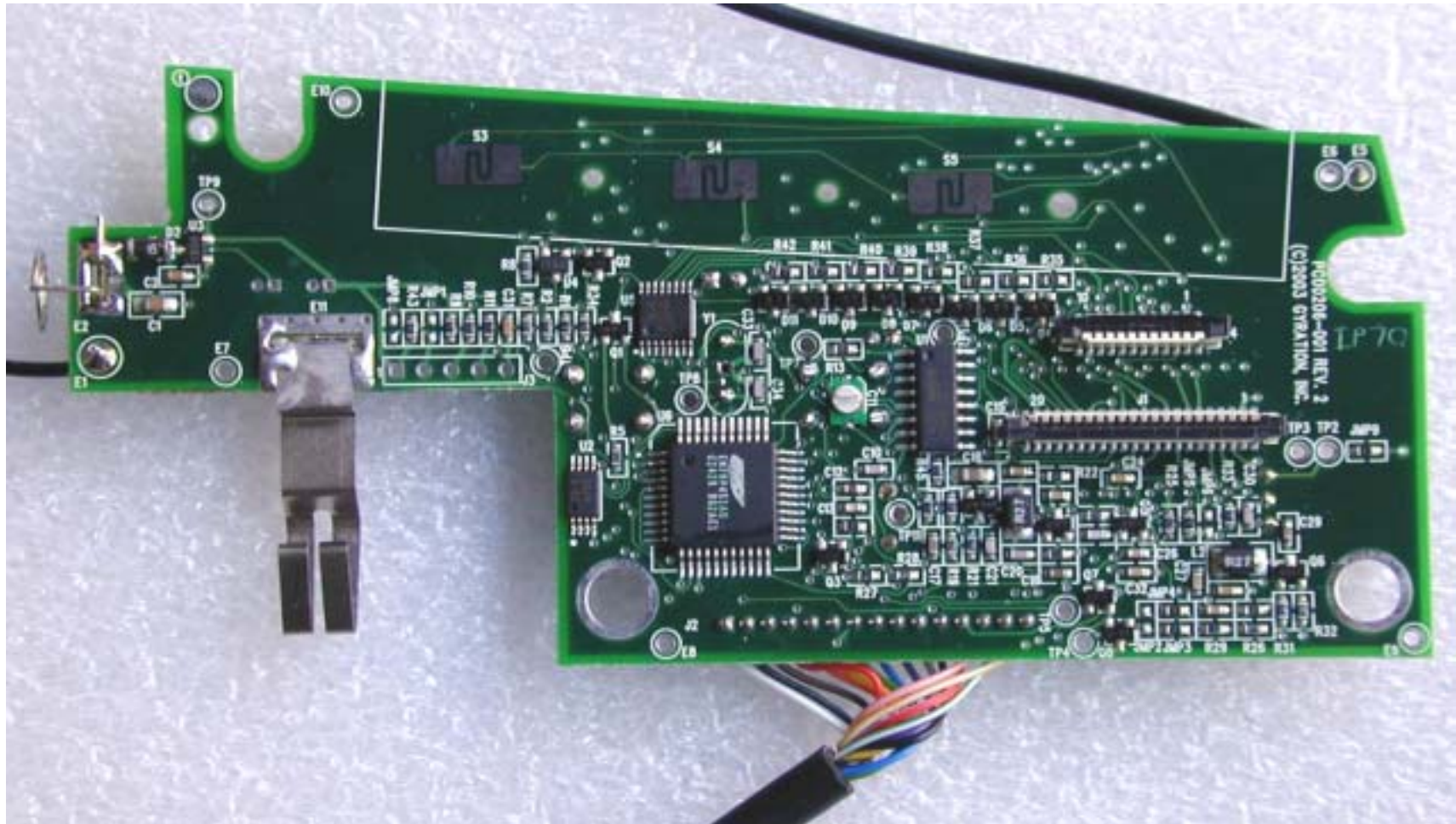
Top Side of Transmitter Board
