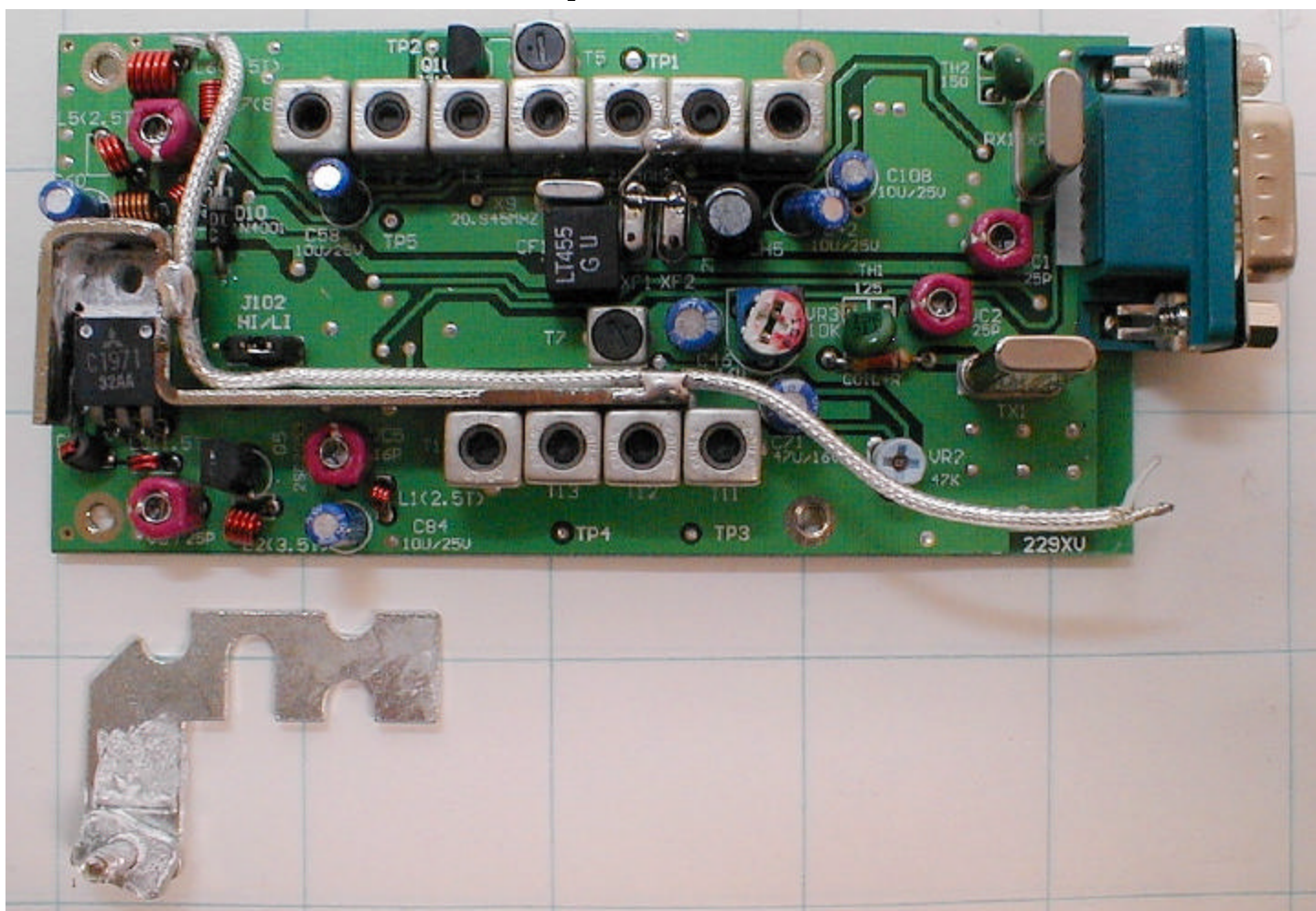
PCB Top with Shield Removed
