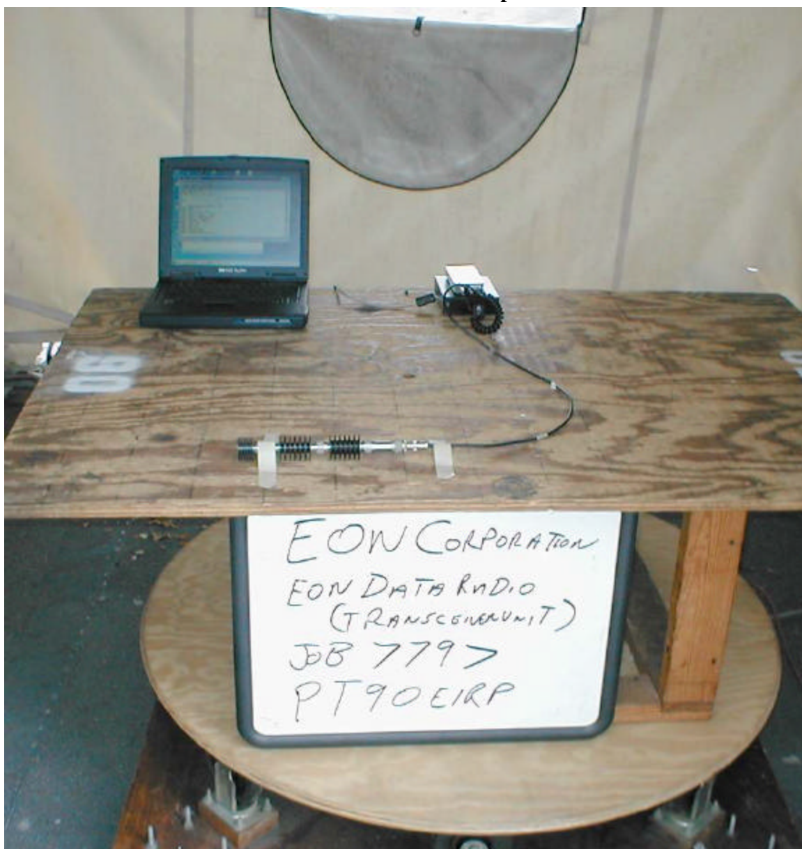
Radiated Emissions Test Setup – Front
