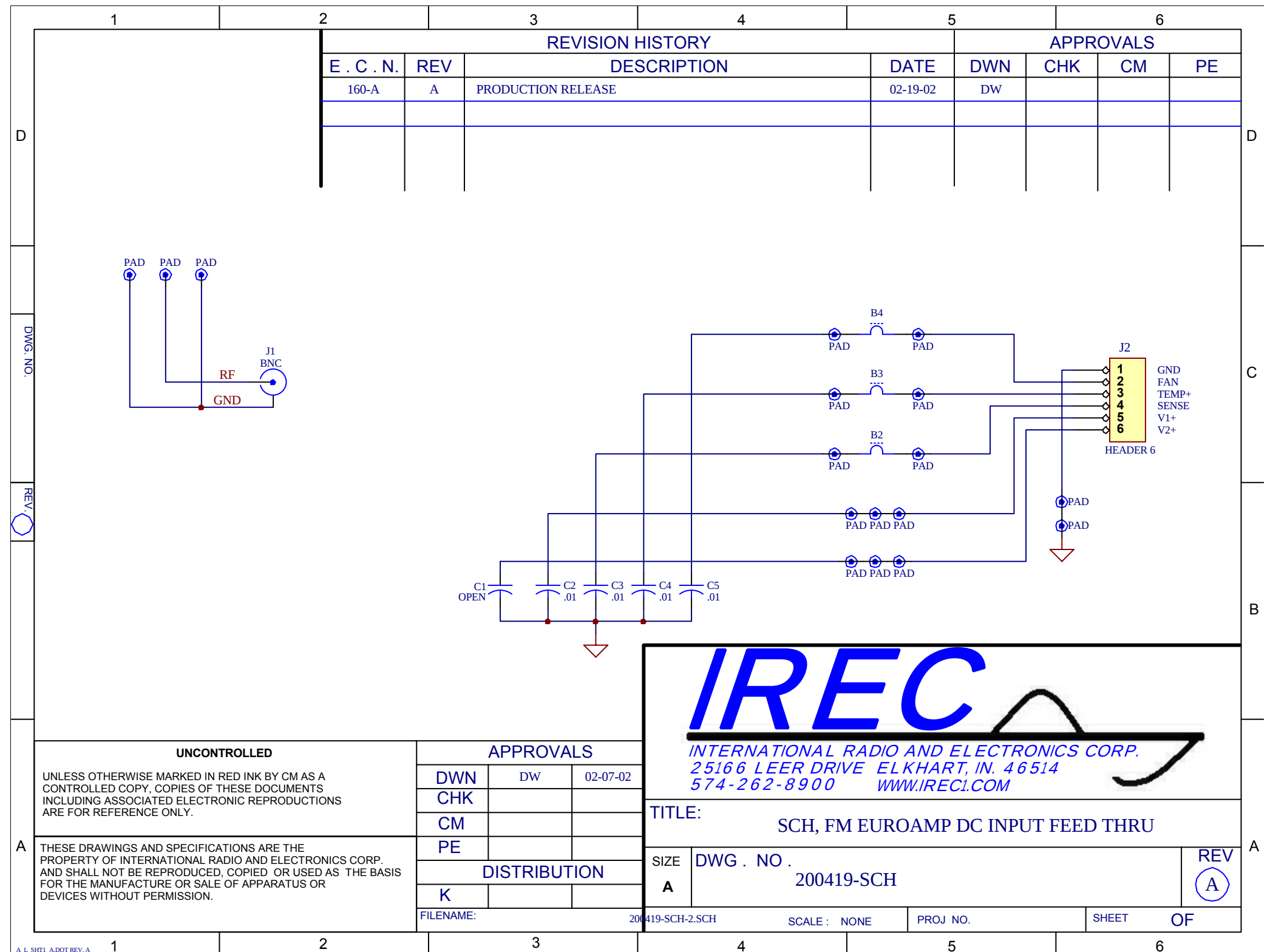
Illustration 6-16 FM Euroamp DC Input Feedthru (Bottom Side)
