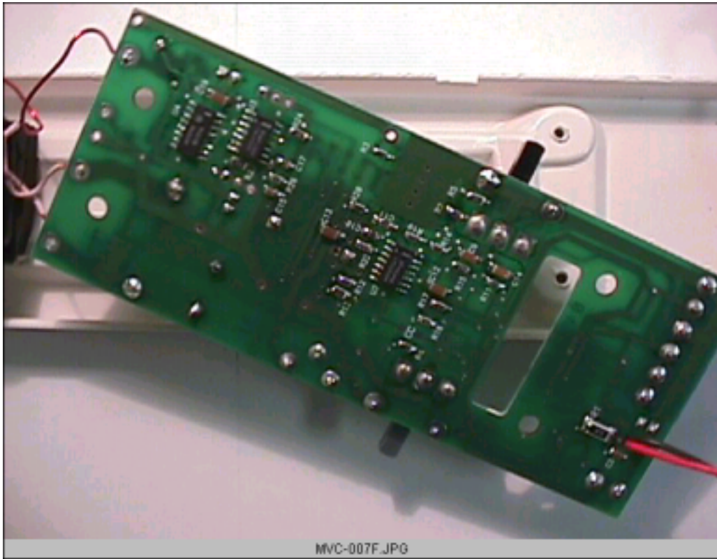
Innovative Control - PCB Transceiver / Foil side
