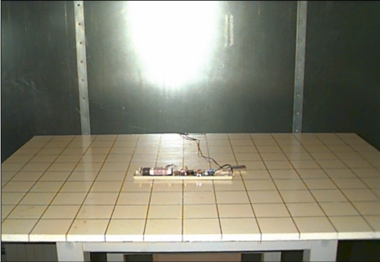
Front view of the Homecare during the Conducted Emissions tests in the Shielded ESD room.
