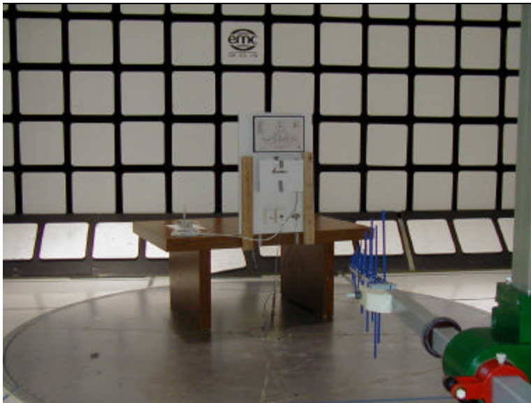
Radiated Emissions Receiver w/ Multiplexer
