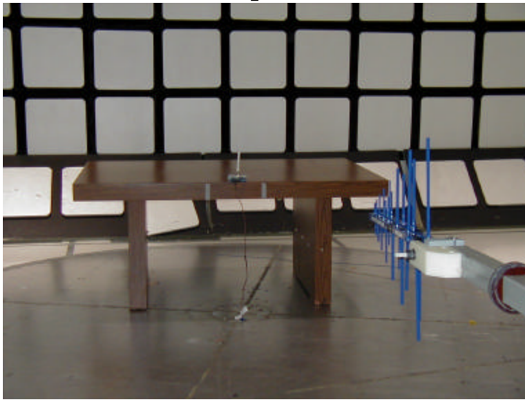
Radiated Emissions Receiver Module Only
