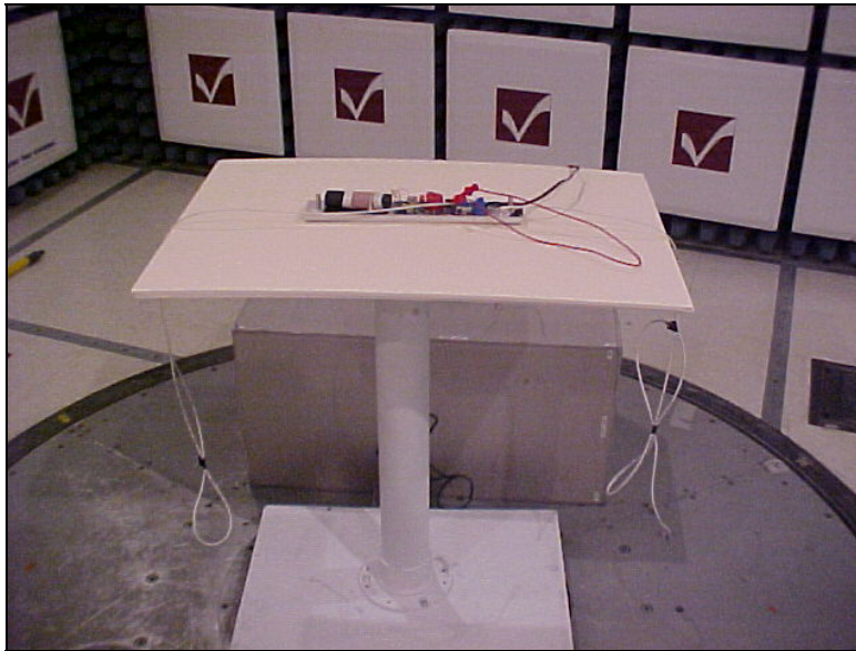
View of the EUT during Radiated Emission Testing in the 3 Meter FCC Listed Chamber, 30 MHz – 1000 MHz & Low Frequency Scans
