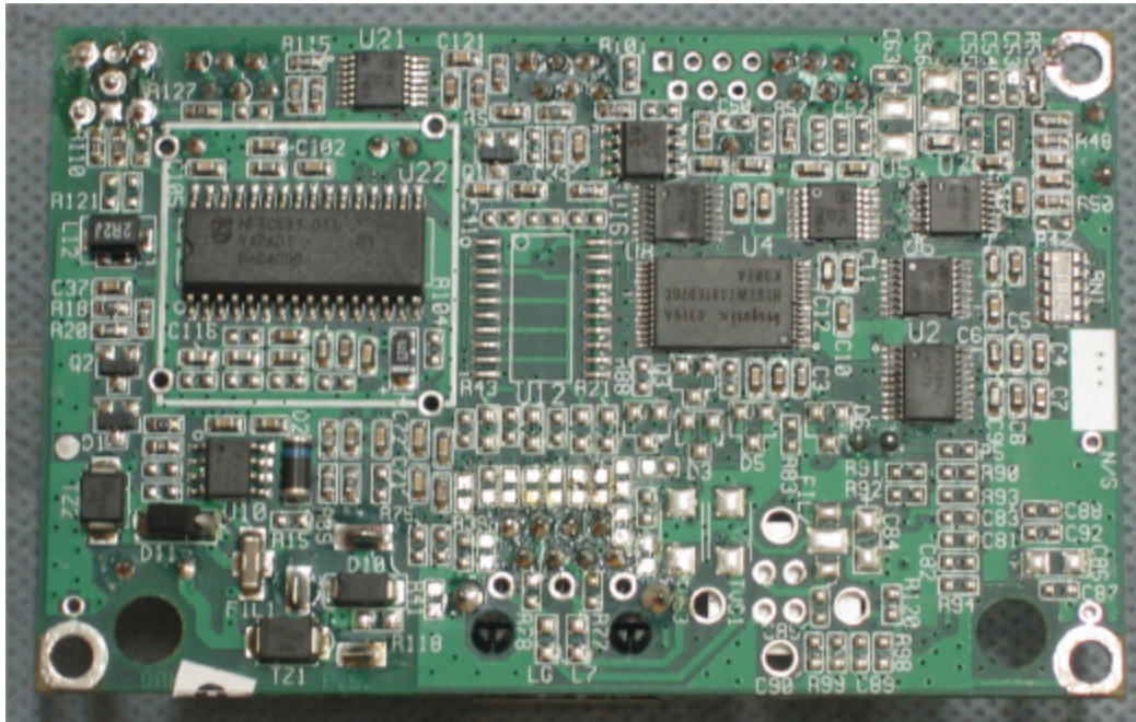
Photograph No.16 Smart card reader SAT5000 (RS232) PCB second side view
