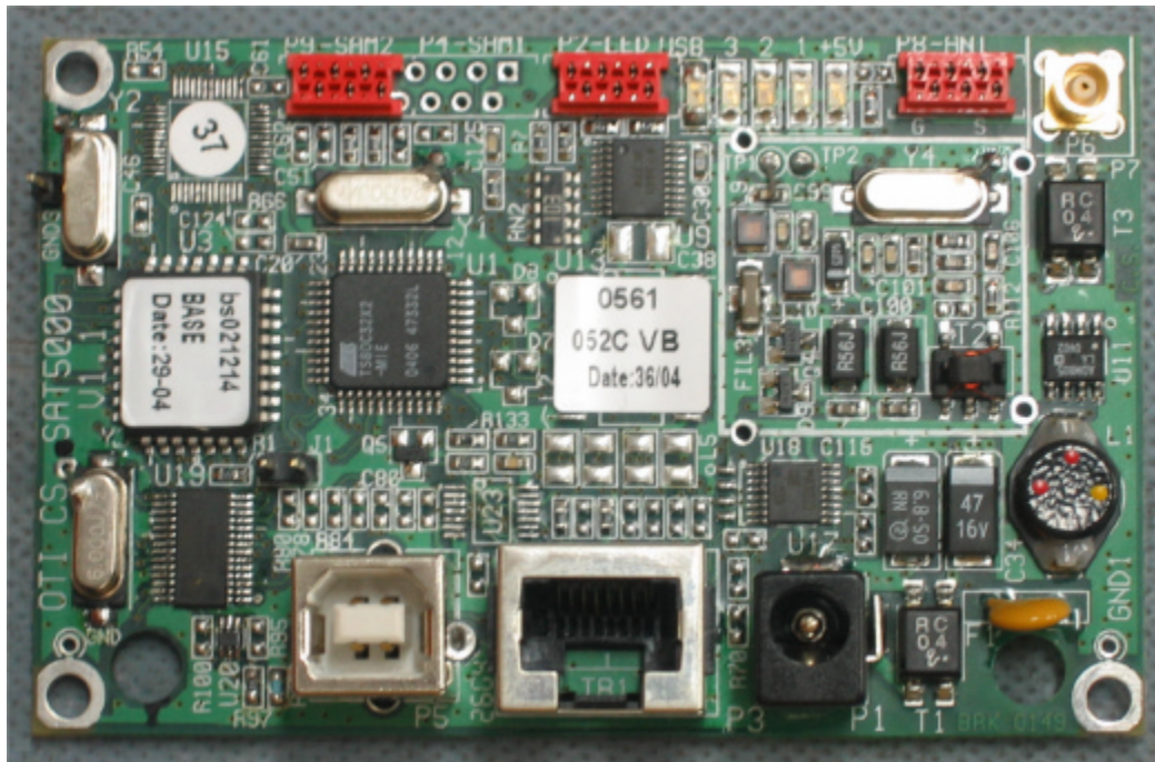
Photograph No.7 Smart card reader SAT5000 (USB) PCB front view
