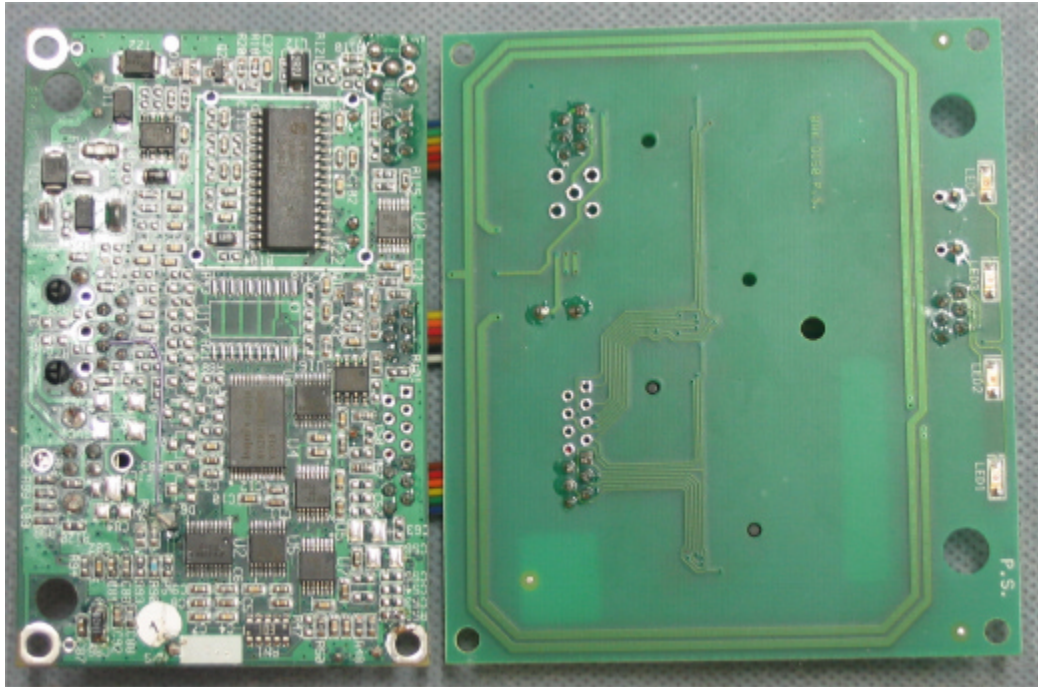
Photograph No4 Smart card reader SAT5000 (USB) PCBs second side view
