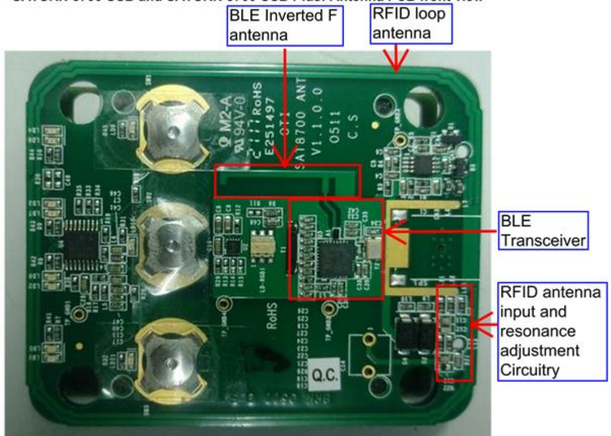
Photograph No.5 SATURN 8700 USB and SATURN 8700 USB Plus: Antenna PCB front view
